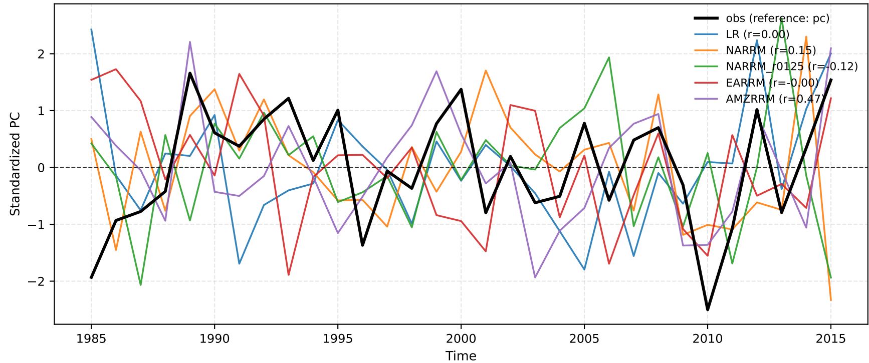
NAO (DJF, 1985-2014) | Standardized pc_proj (projected onto OBS EOF)
