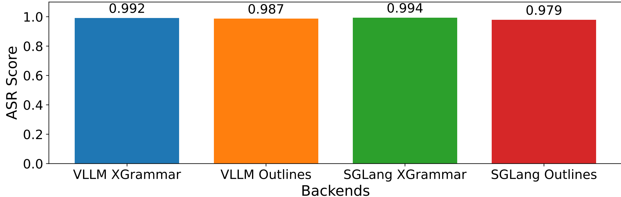
ASR - Enum Attack on Llama-3.1-8B with different backends
