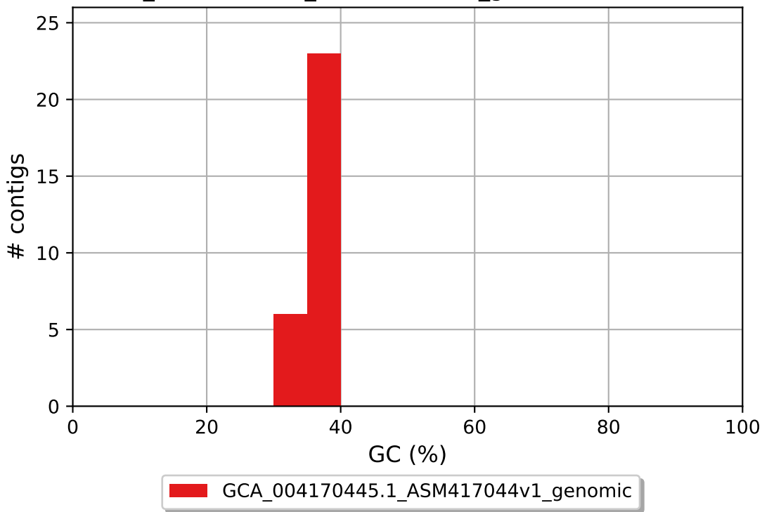
GCA_004170445.1_ASM417044v1_genomic GC content
