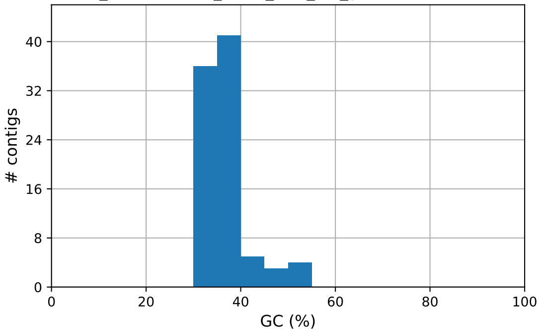
GCA_009771035.1_CNRS_Lalb_1.0_genomic GC content
