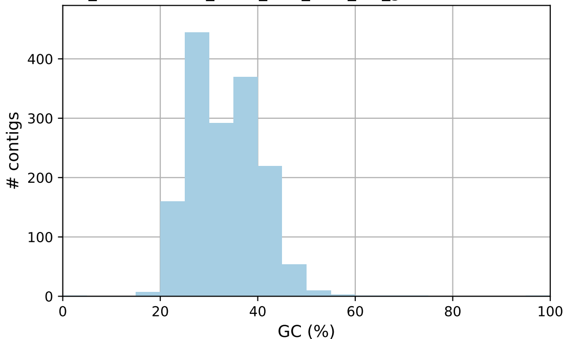
GCF_024323335.1_CAAS_Psat_ZW6_1.0_genomic GC content
