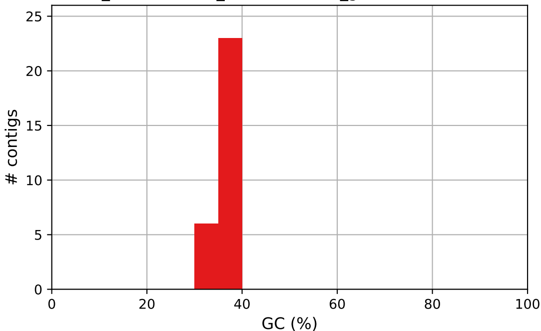
GCA_004170445.1_ASM417044v1_genomic GC content
