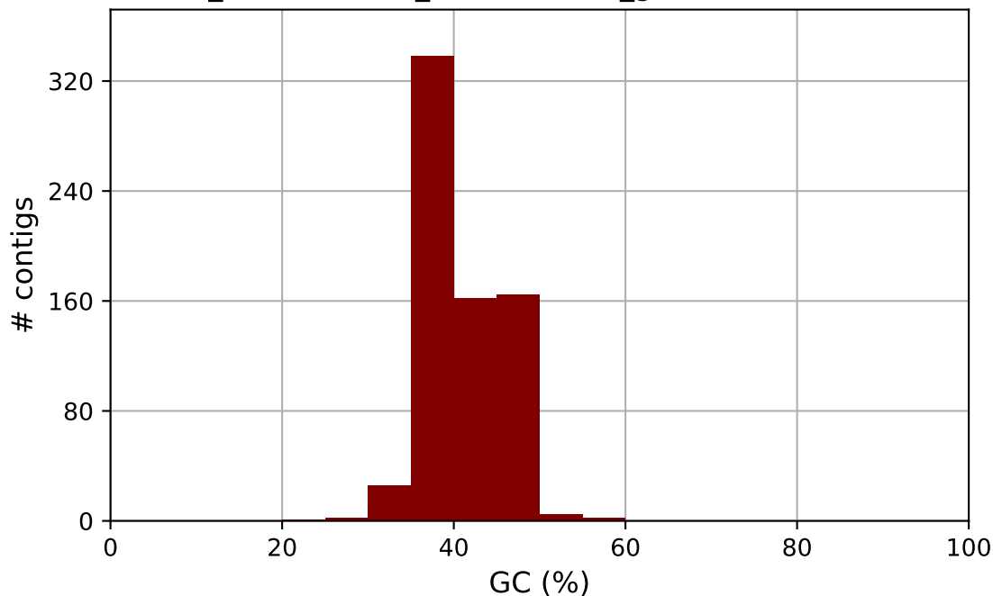
GCF_000715075.1_ASM71507v2_genomic GC content
