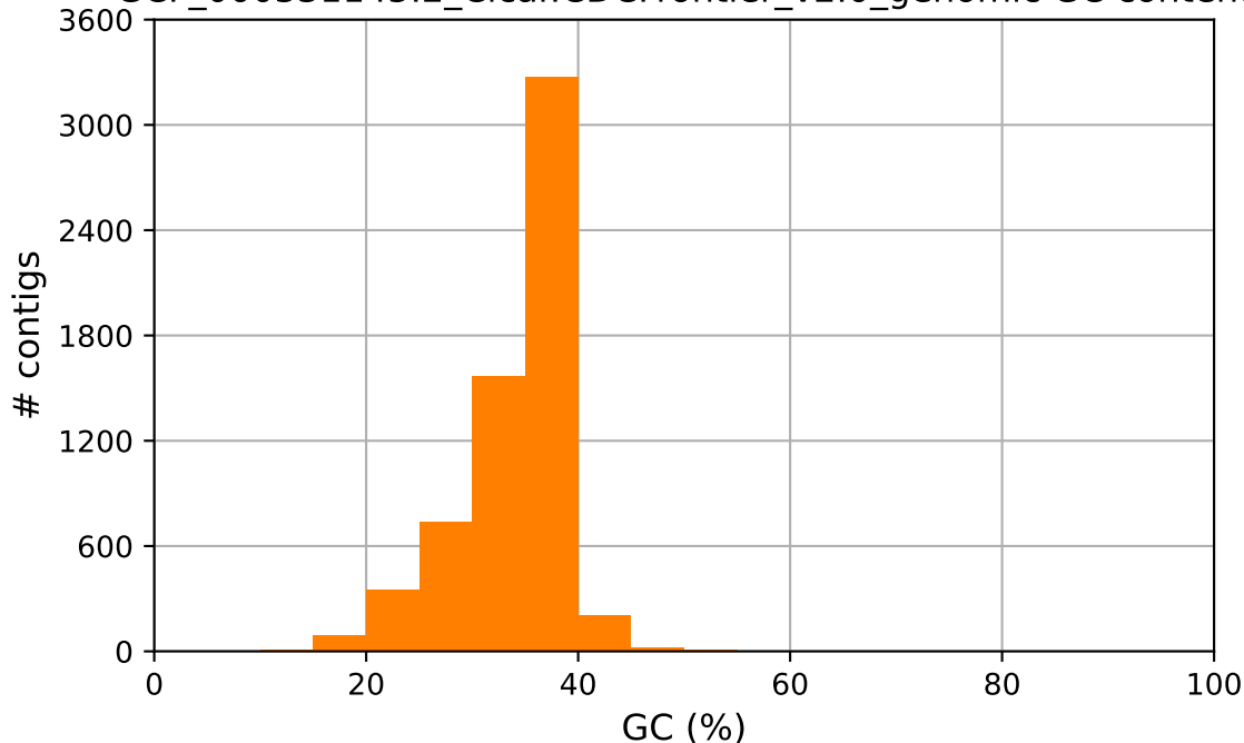
GCF_000331145.2_Cicar.CDCFrontier_v2.0_genomic GC content
