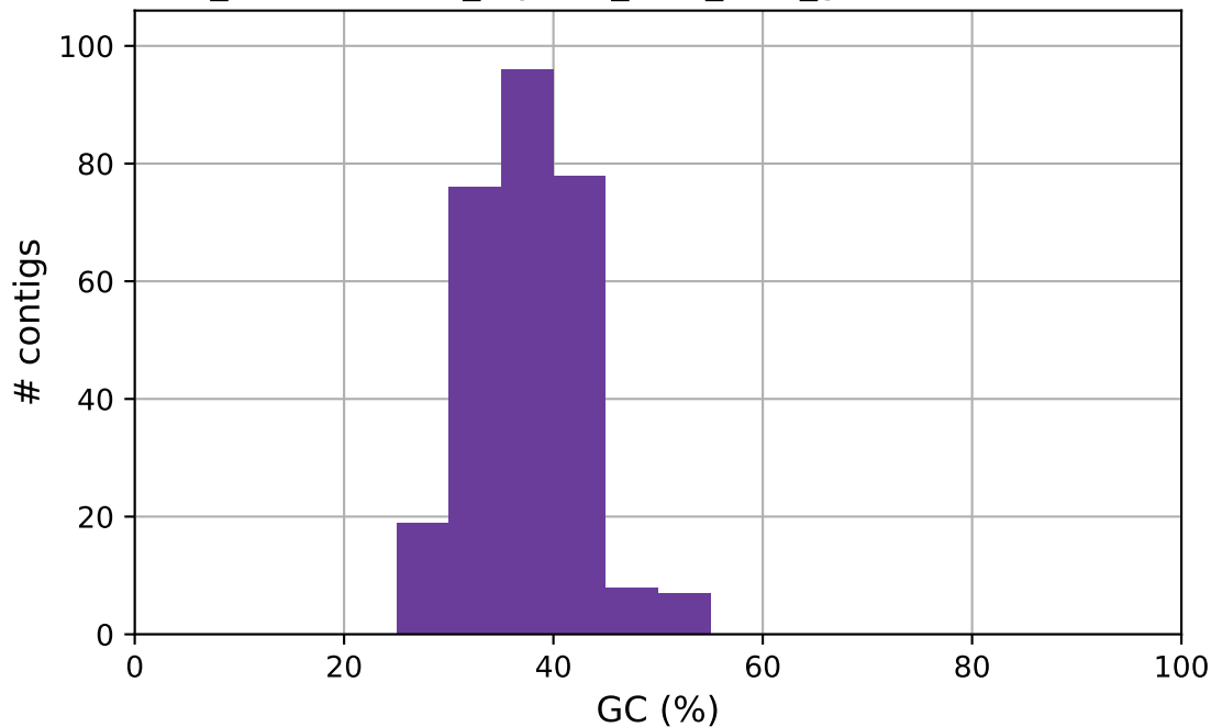
GCF_000004515.6_Glycine_max_v4.0_genomic GC content
