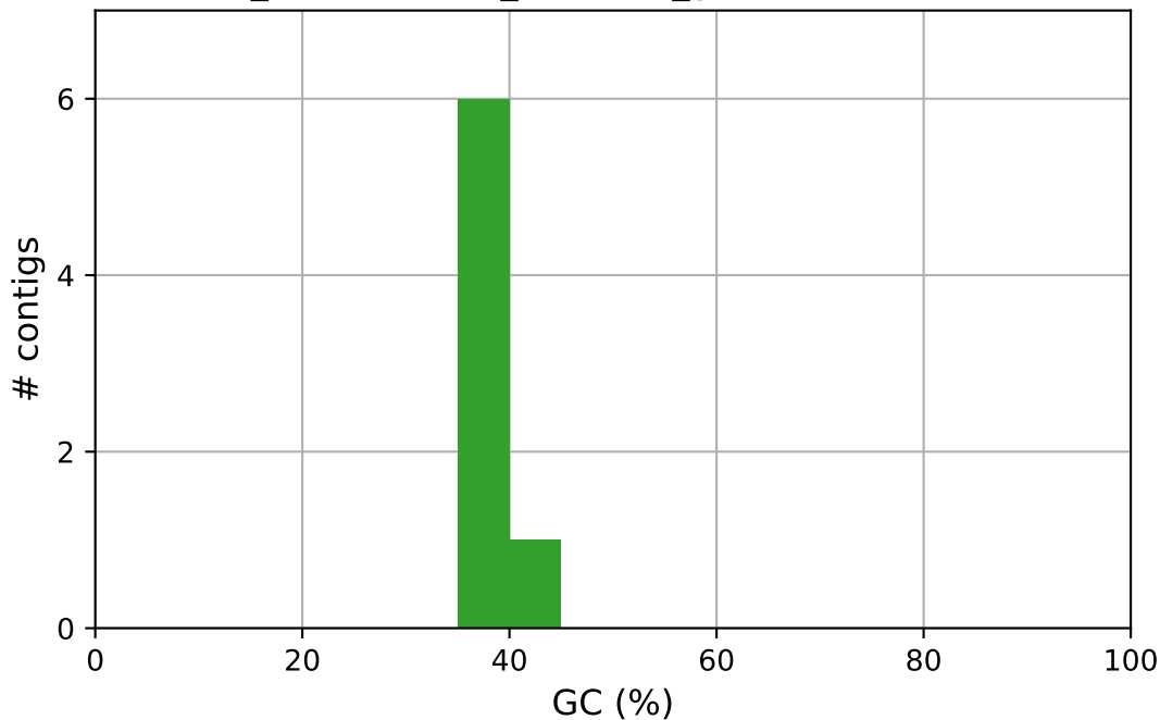
GCF_000001735.4_TAIR10.1_genomic GC content
