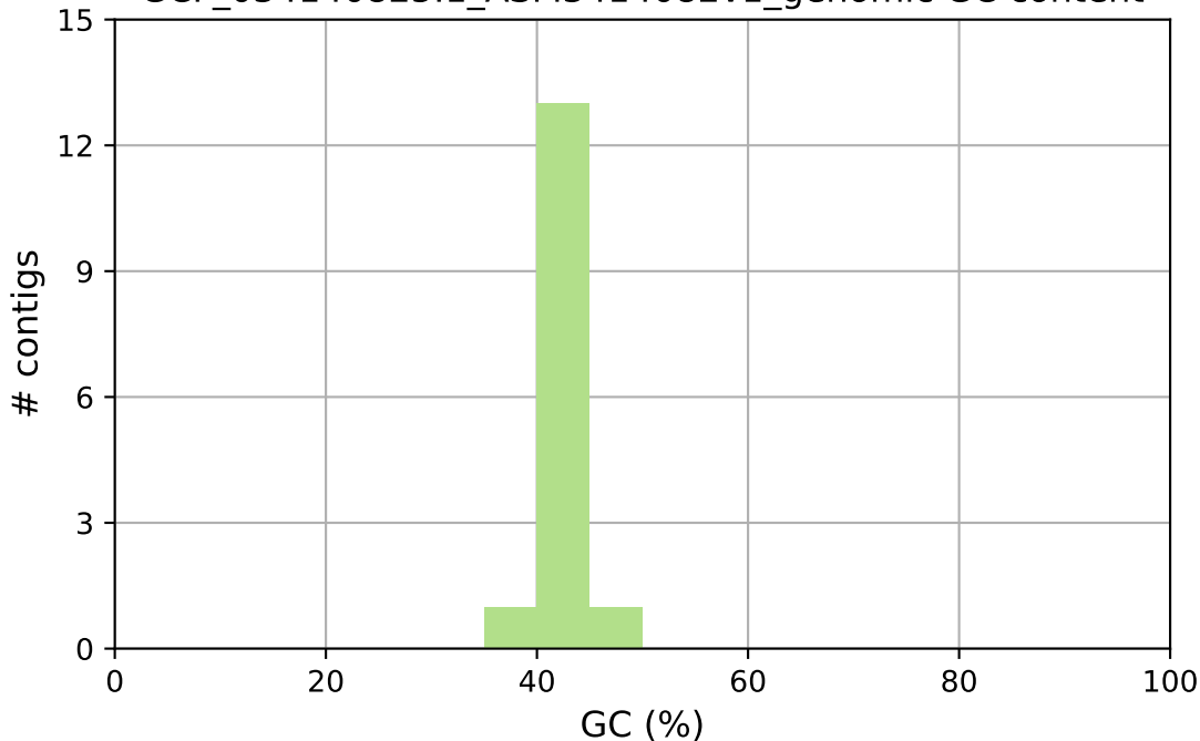
GCF_034140825.1_ASM3414082v1_genomic GC content
