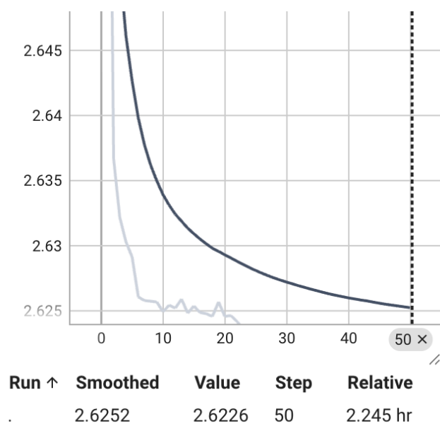
Train/EpochLoss
