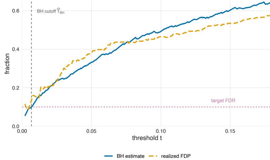
FIGURE 5.4. A single simulated path of the realized FDP and the BH estimator mt/R(t) . The estimator need not dominate the realized FDP pointwise; the BH theorem is an expectation statement at the selected cutoff. The gray vertical line marks the canonical BH cutoff \hat{T}_{\text{BH}} = \hat{q}k/m . Here m = 700 , q = 0.10 , and 90 one-sided Gaussian signals have mean 2.45.
