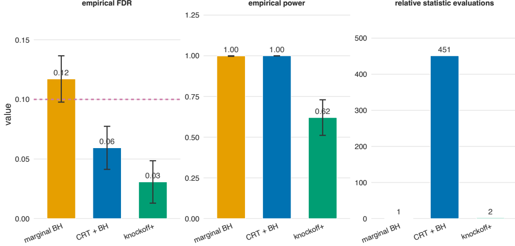
FIGURE 9.5. A Gaussian model-X simulation with n = 220 , p = 40 , 14 signals of size 1, AR(1) correlation \rho = 0.5 , and FDR target q = 0.10 . The empirical FDR and empirical power are averaged over 64 independent simulated data sets; their vertical bars are pointwise 95 percent normal simulation intervals. CRT uses B = 450 conditional resamples per feature, while knockoff+ uses one knockoff copy and a signed marginal-correlation statistic. The right panel shows relative statistic evaluations, not wall-clock time.
