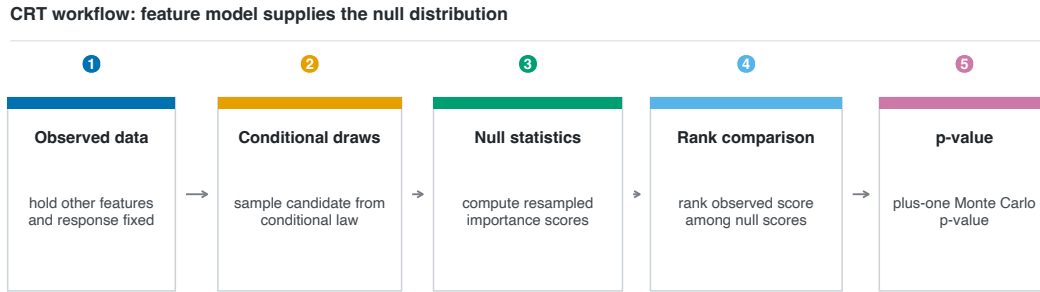
FIGURE 9.1. Conditional randomization test. The conditional feature law, not a model for Y | X , supplies the null distribution. The final p-value uses the plus-one Monte Carlo correction.
