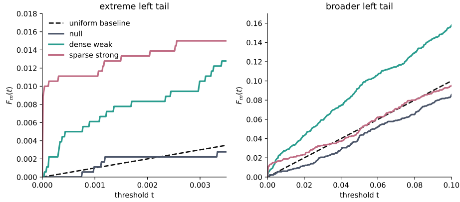
FIGURE 1. Left-tail empirical CDFs of one-sided p-values under a null model, a dense weak alternative, and a sparse stronger alternative. In this stylized draw, m = 1800 , the dense weak case shifts 360 coordinates by 1.0, and the sparse strong case shifts 24 coordinates by 4.2. The diagonal is the uniform baseline. The extreme-left panel shows the sparse alternative creating the sharpest bump very near zero; the broader-left panel shows the dense weak alternative lifting the CDF over a wider range.
