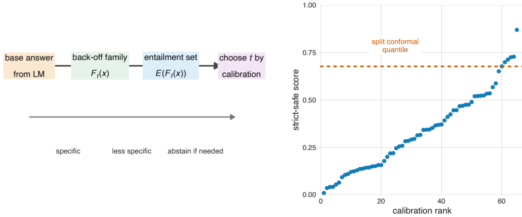
FIGURE 13.6. Reference-relative factuality. A back-off family produces less specific answers whose entailment sets are easier for the reference to satisfy. Split conformal calibration chooses the back-off threshold from strict-safe scores.
