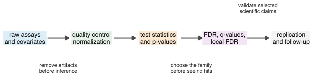
FIGURE 13.1. A large-scale genomic analysis pipeline. Multiple-testing methods enter after the measurement scale and test family have been fixed. The selected discoveries then need replication, biological validation, or a second-stage inferential analysis.
