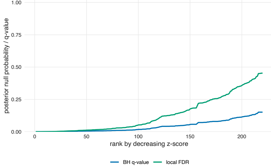
FIGURE 5. Local FDR and BH q-values for the most significant simulated z-scores. Local FDR ranks individual cases by posterior null probability, while q-values summarize the tail set that would be reported at each rank.
