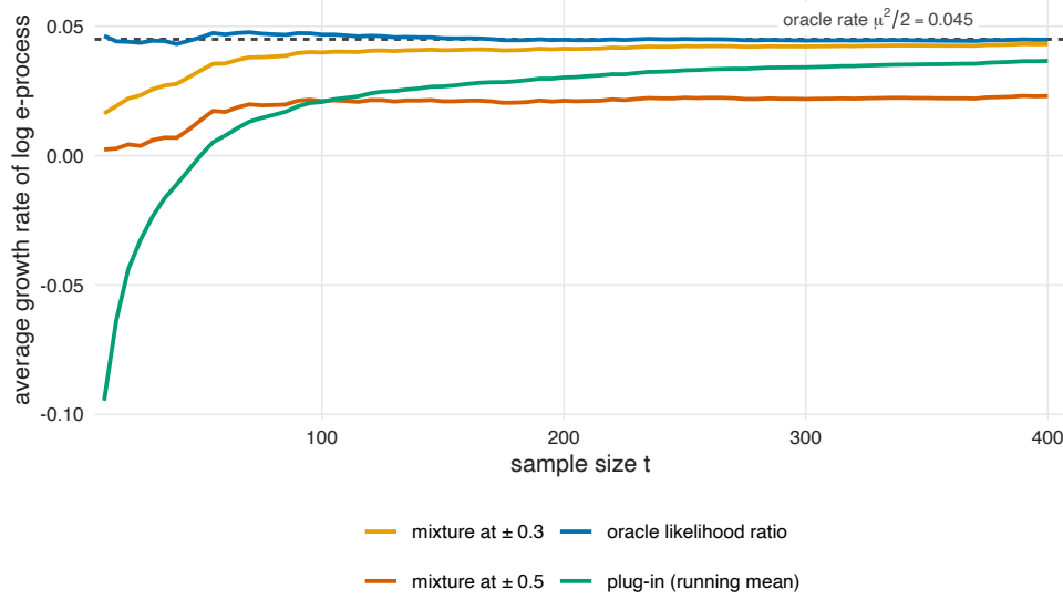
FIGURE 4. Average growth rate t^{-1}\mathbb{E}_Q[\log M_t] of four e-processes for H_0 : \mu = 0 , estimated from 300 simulated N(0.3, 1) sequences of length 400. The oracle likelihood ratio that knows \mu = 0.3 sits at the rate \mu^2/2 = 0.045 ; the predictable plug-in with the running-mean estimate climbs toward the same rate; the two-point mixture at \pm 0.3 approaches it; and the mixture at \pm 0.5 settles near its theoretical rate \delta\mu - \delta^2/2 = 0.025 .
