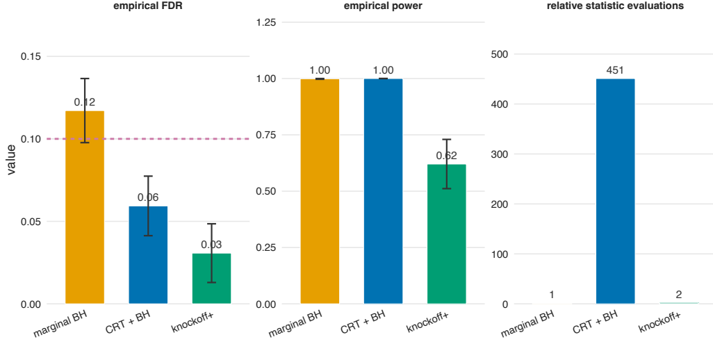
FIGURE 9.5. A Gaussian model- X simulation with n = 220 , p = 40 , 14 signals of size 1, AR(1) correlation \rho = 0.5 , and FDR target q = 0.10 . The empirical FDR and empirical power are averaged over 64 independent simulated data sets; their vertical bars are pointwise 95 percent normal simulation intervals. CRT uses B = 450 conditional resamples per feature, while knockoff+ uses one knockoff copy and a signed marginal-correlation statistic. The right panel shows relative statistic evaluations, not wall-clock time.
