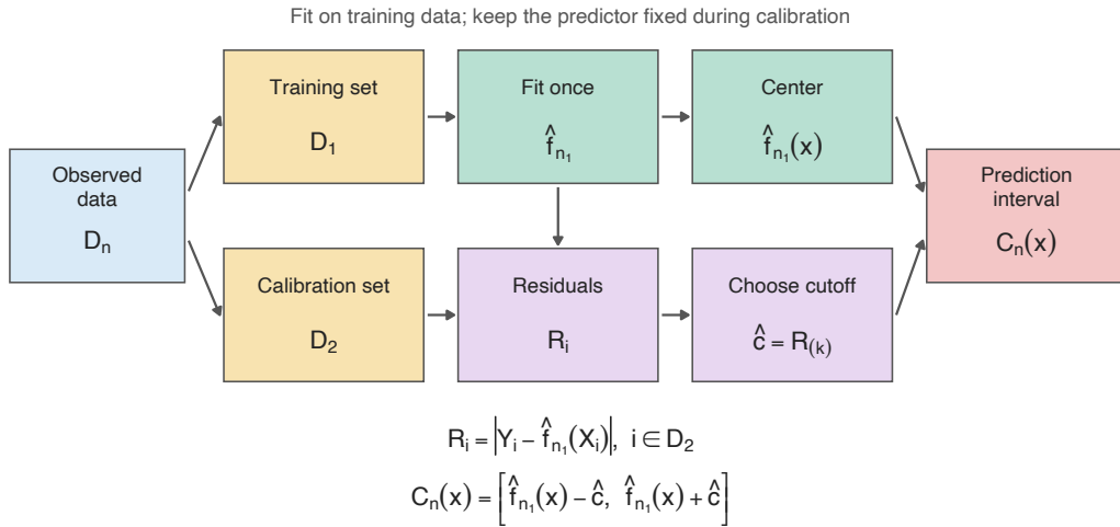
FIGURE 10.2. Split conformal prediction with absolute residuals. Split D_n into a proper training set D_1 of size n_1 and a calibration set D_2 of size n_2 . Fit \hat{f}_{n_1} on D_1 ; the same fitted predictor supplies the interval center and the residuals on D_2 . “Choose cutoff” means take the k th smallest calibration residual, with k = \lceil (1 - \alpha)(n_2 + 1) \rceil , setting \hat{c} = \infty if k = n_2 + 1 . The interval combines this cutoff with the center at x . Coverage follows from exchangeability of the calibration and future test scores conditional on D_1 .
