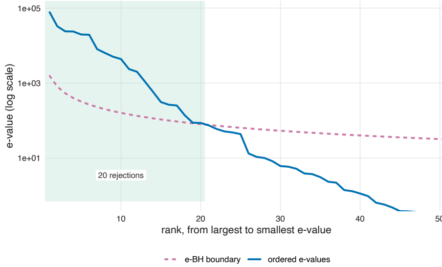
FIGURE 8.5. The e-BH rule in one simulated family of m = 160 hypotheses. Each hypothesis has n = 12 independent N(\mu_i, 1) observations; data are also independent across hypotheses. The 124 null means are zero and the 36 nonnull means are \theta = 0.9 . Writing Z_i = \sqrt{n} \bar{X}_i , we compute the likelihood-ratio e-value E_i = \exp\{\theta\sqrt{n} Z_i - n\theta^2/2\} for testing \mu_i = 0 against \mu_i = \theta . At target q = 0.10 , e-BH compares the ordered e-values with m/(qk) over all 160 ranks; the plot shows the first 50. The largest crossing rank is \hat{k} = 20 . All top 20 hypotheses are rejected, including any earlier ranks whose values lie below their own rankwise boundaries.
