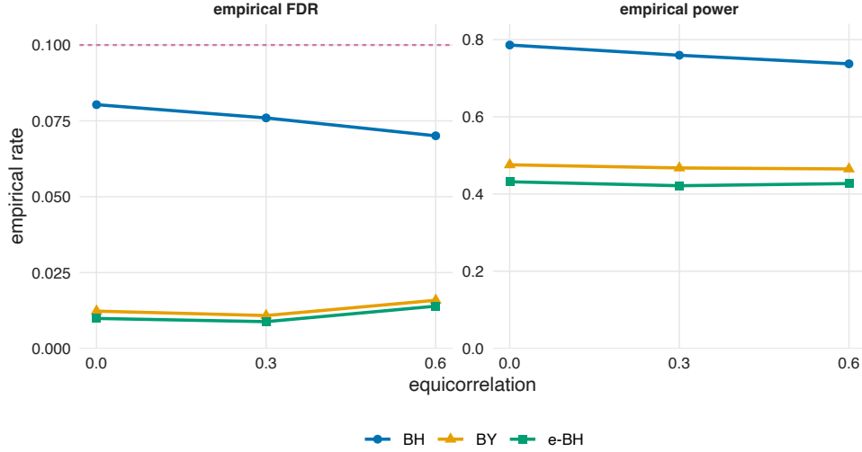
FIGURE 8.6. Empirical FDR and empirical power with m = 400 hypotheses, 80 nonnulls, equicorrelated Gaussian test statistics based on n = 20 observations with working effect \theta = 0.65 , 650 independent simulation runs, correlations \rho \in \{0, 0.3, 0.6\} , and q = 0.10 . The e-values are Gaussian likelihood ratios \exp\{\theta\sqrt{n}Z - n\theta^2/2\} . The lesson is not that e-BH is always more powerful; it is that e-BH's proof uses an e-value moment condition rather than a p-value dependence condition.
