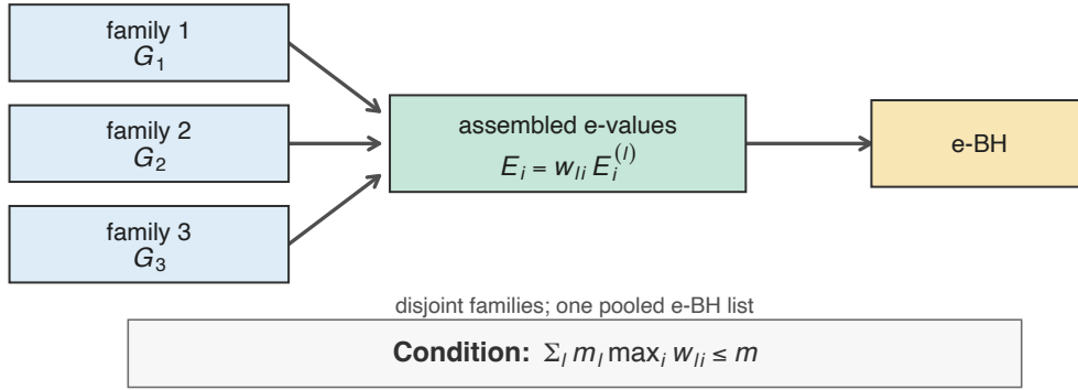
FIGURE 8. Combining evidence from several procedures on the same hypotheses and assembling evidence from disjoint datasets. In assembling, the main output is one pooled e-BH list; family-level aggregate bounds also justify separate family lists when reported. The max-weight conditions protect against unknown true-null placement.
