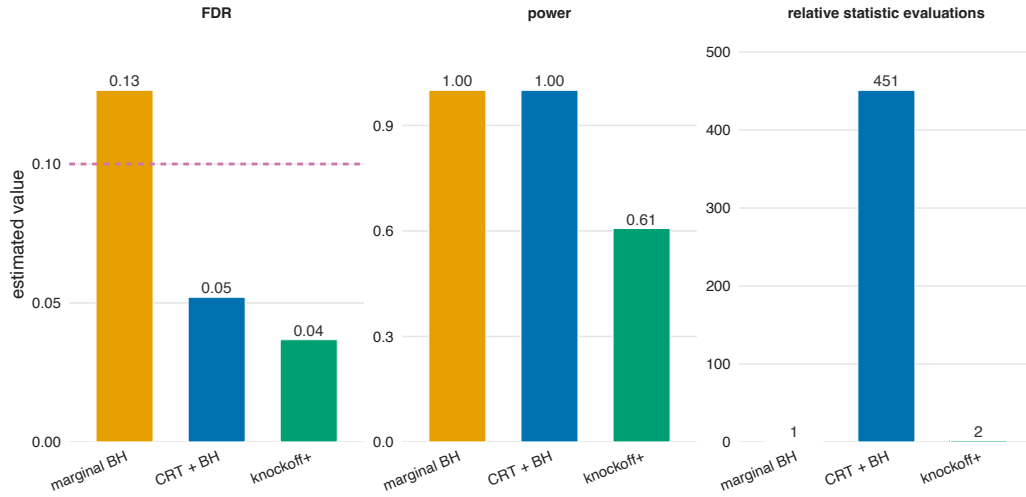
FIGURE 9.5. A small Gaussian model-X simulation with correlated features. CRT uses B = 450 conditional resamples per feature; knockoff+ uses one knockoff copy and a signed marginal-correlation statistic. The right panel shows relative statistic evaluations, not wall-clock time.
