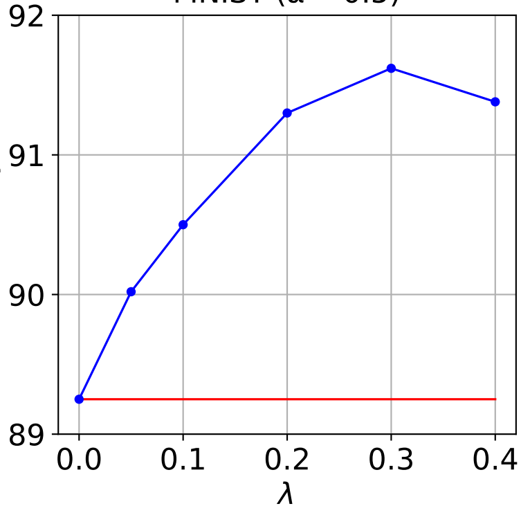
MNIST ( \alpha = 0.5 )
