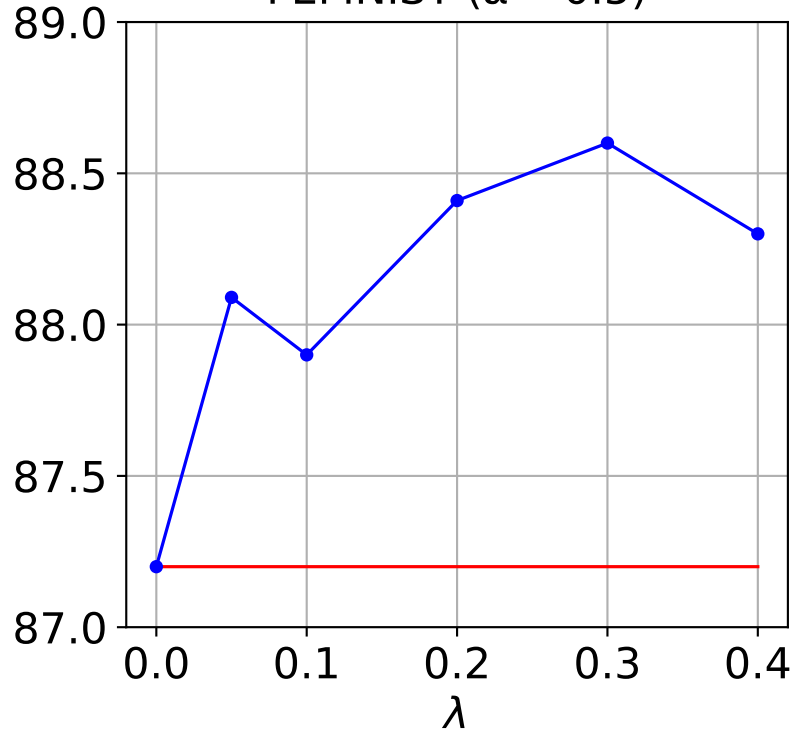
FEMNIST ( \alpha = 0.5 )
