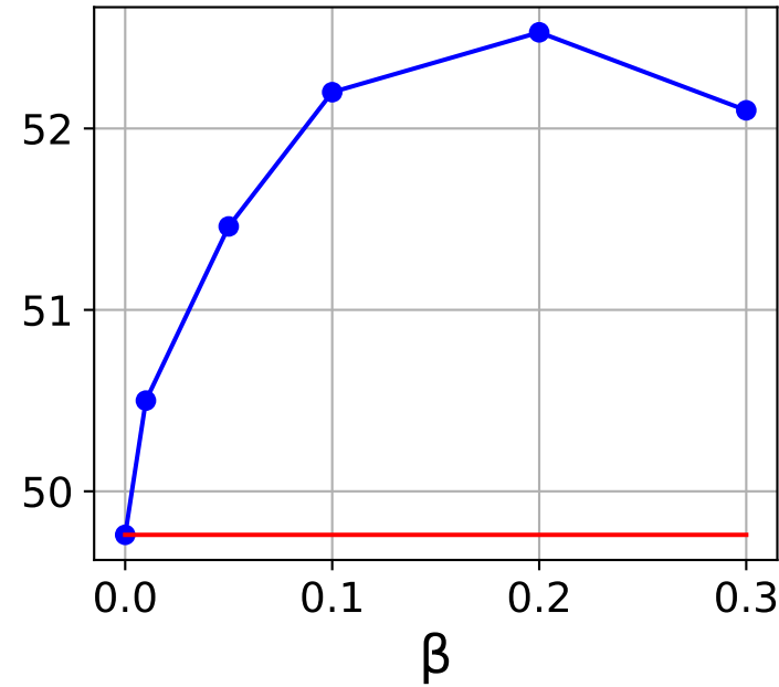
CIFAR100 ( \alpha = 0.05 )
