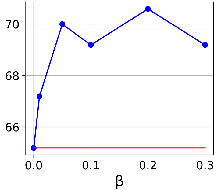
CIFAR10 ( \alpha = 0.1 )
