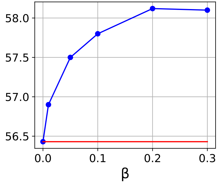
CIFAR100 ( \alpha = 0.1 )
