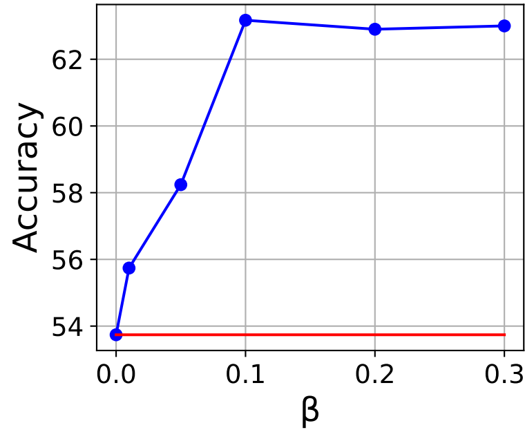
CIFAR10 ( \alpha = 0.05 )
