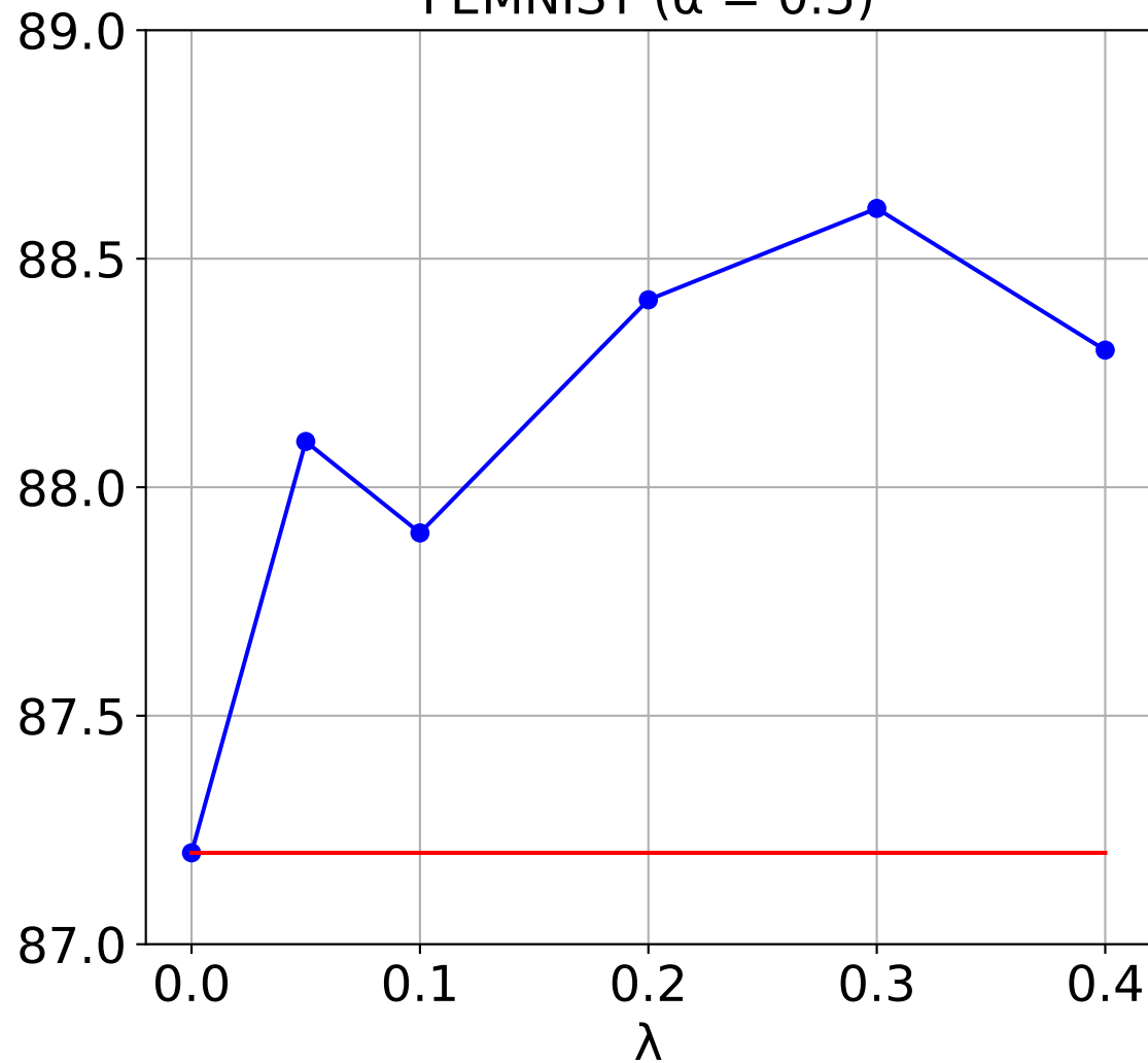
FEMNIST ( \alpha = 0.5 )
