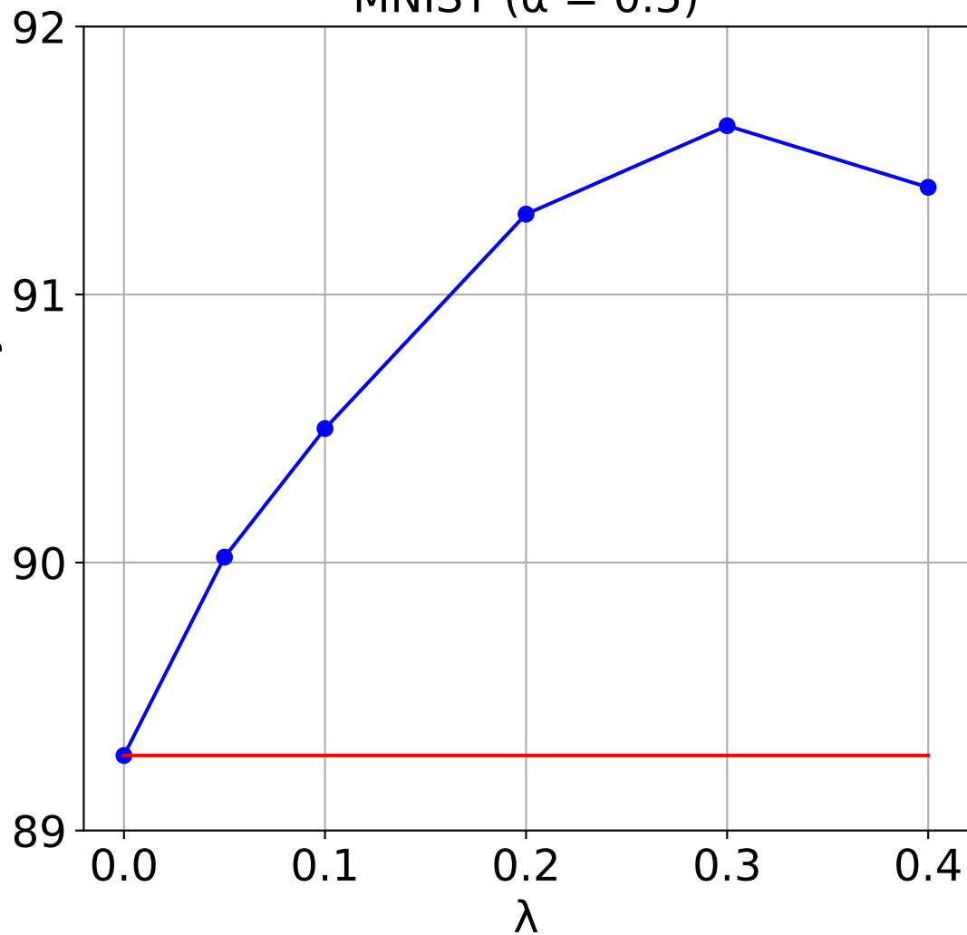
MNIST ( \alpha = 0.5 )
