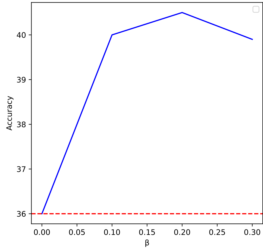
TinyImageNet ( \alpha = 0.05 )
