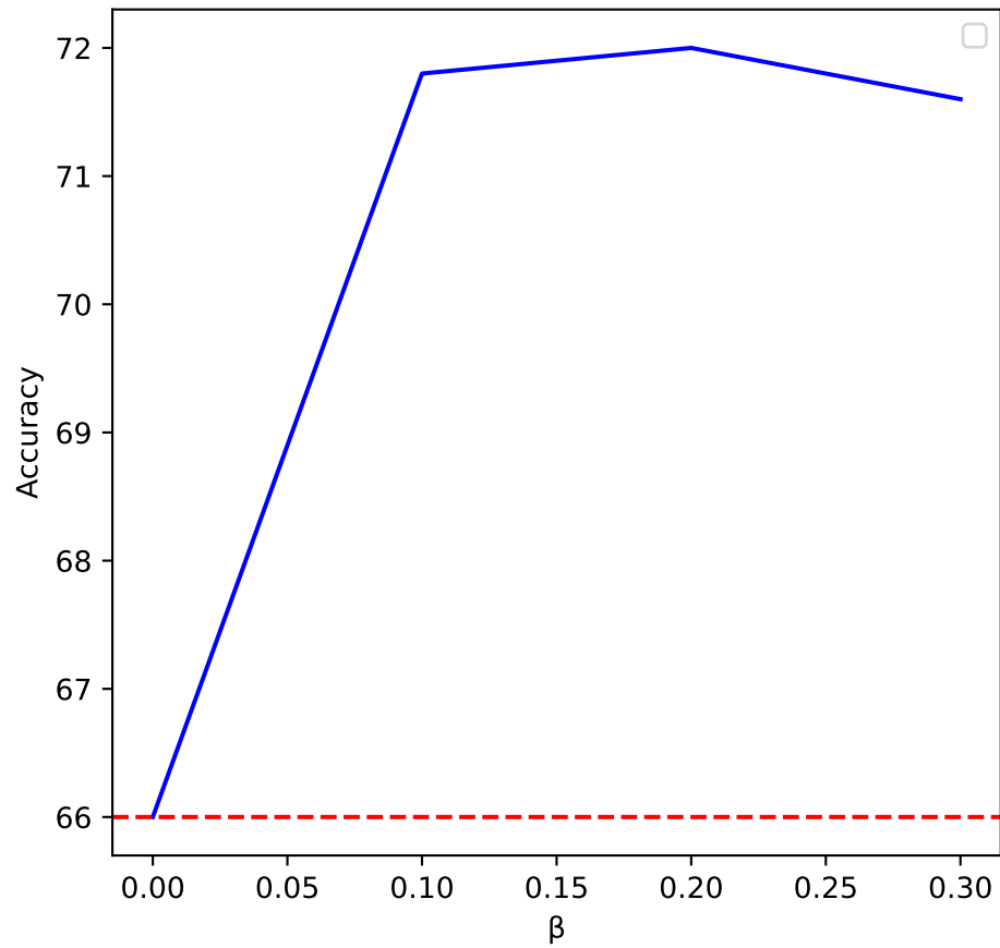
CIFAR10 ( \alpha = 0.05 )
