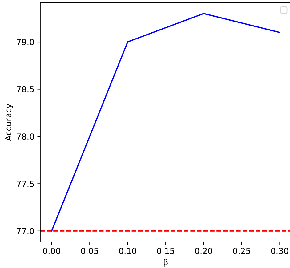
CIFAR10 ( \alpha = 0.1 )
