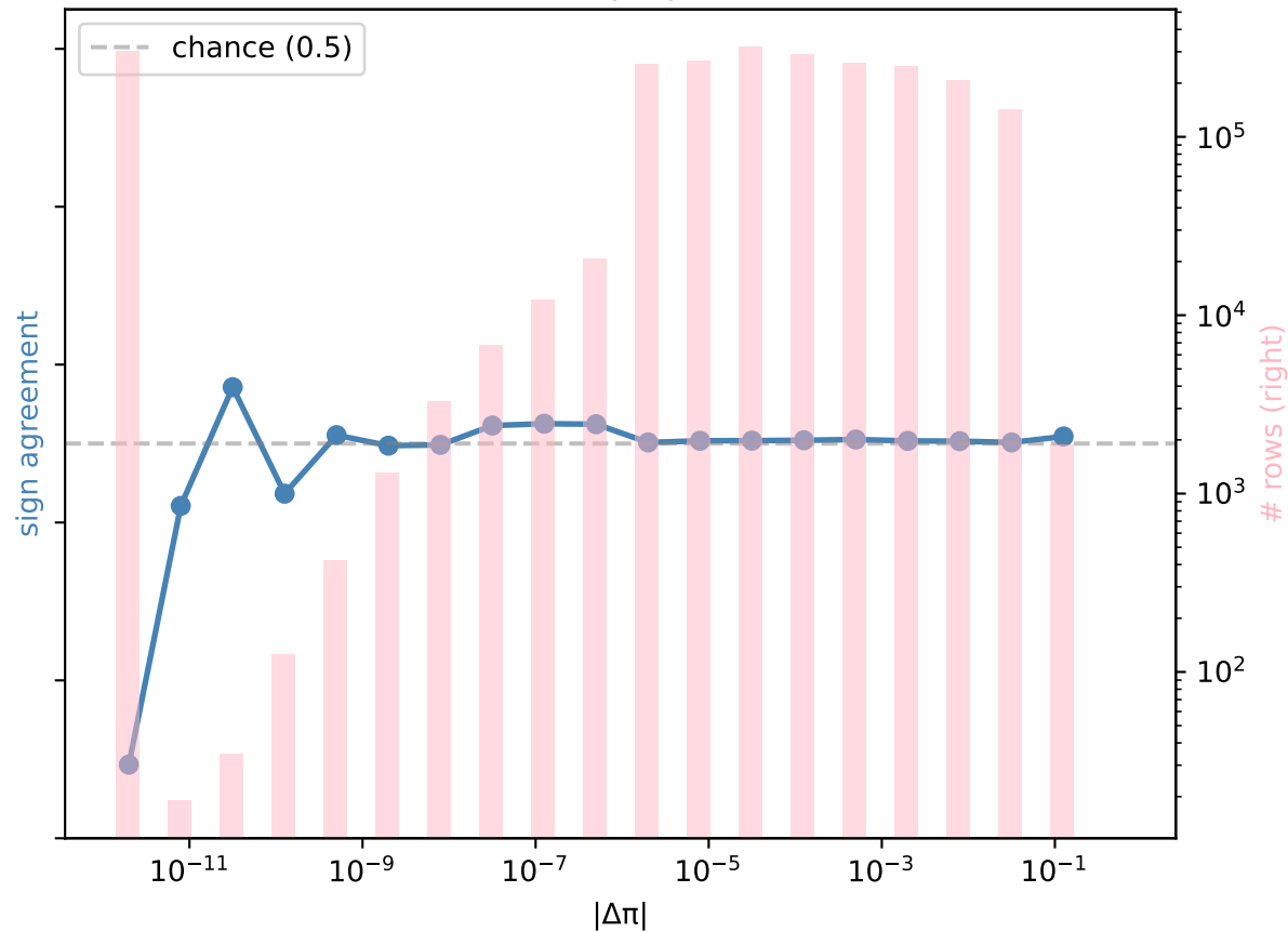
sign agreement vs |\Delta\pi| : sampled u only
