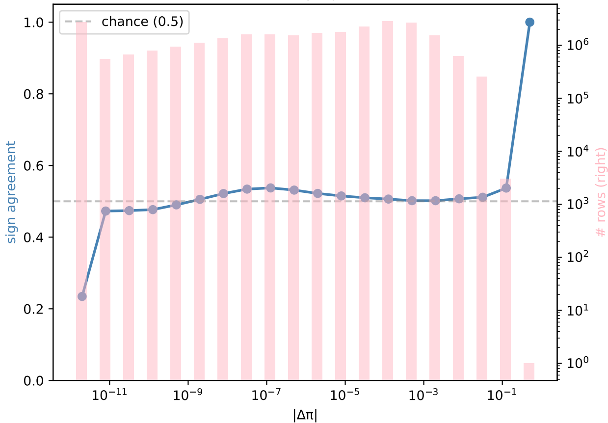
sign agreement vs |\Delta\pi| : all candidates
