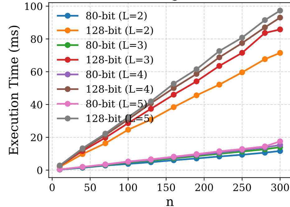
(f) Time Cost of Merge (extended mode)
