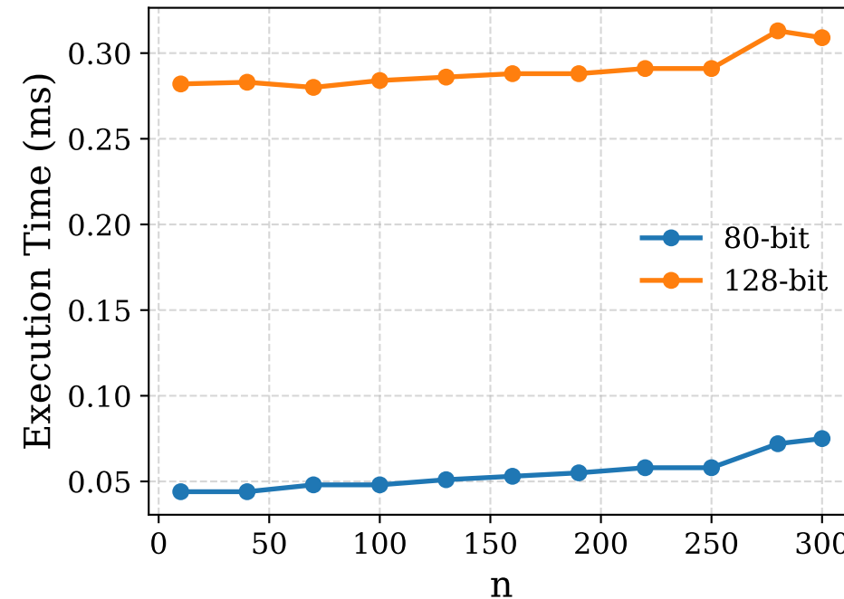
(c) Time Cost of Remove
