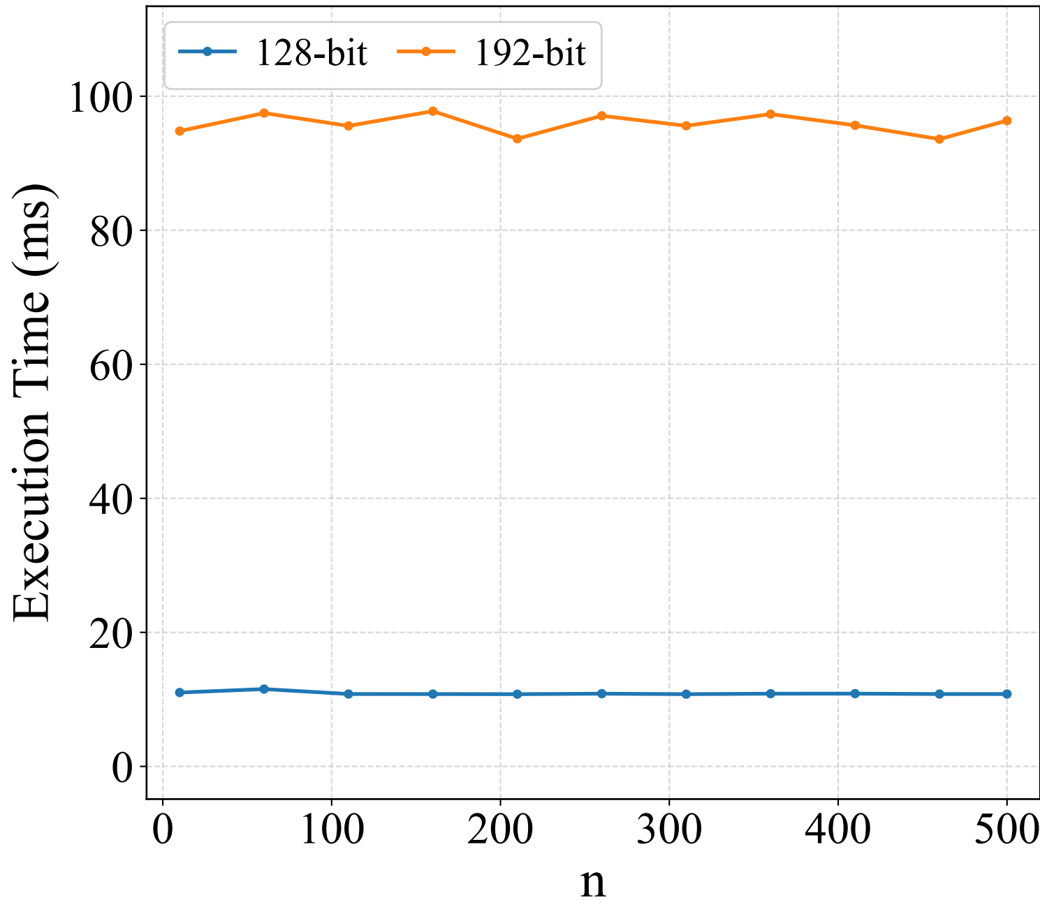
(h) Time Cost of Decap
