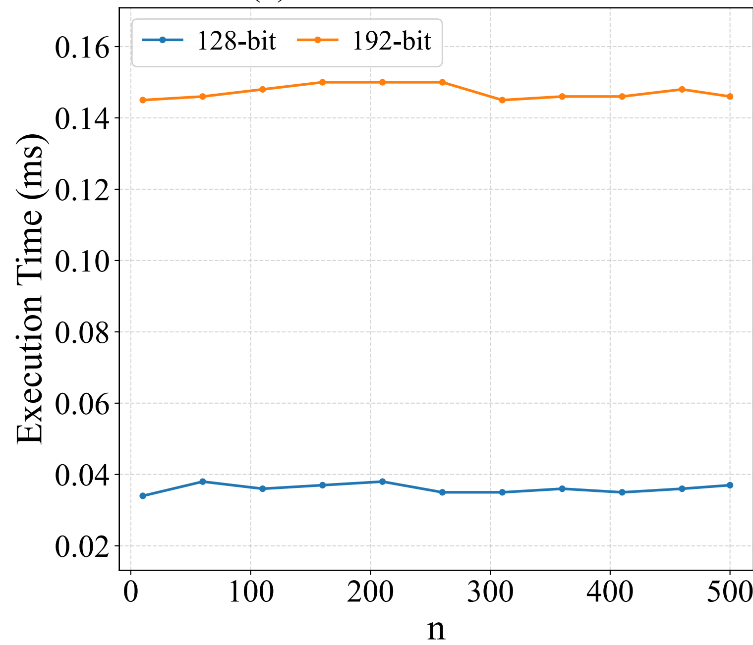
(c) Time Cost of Remove
