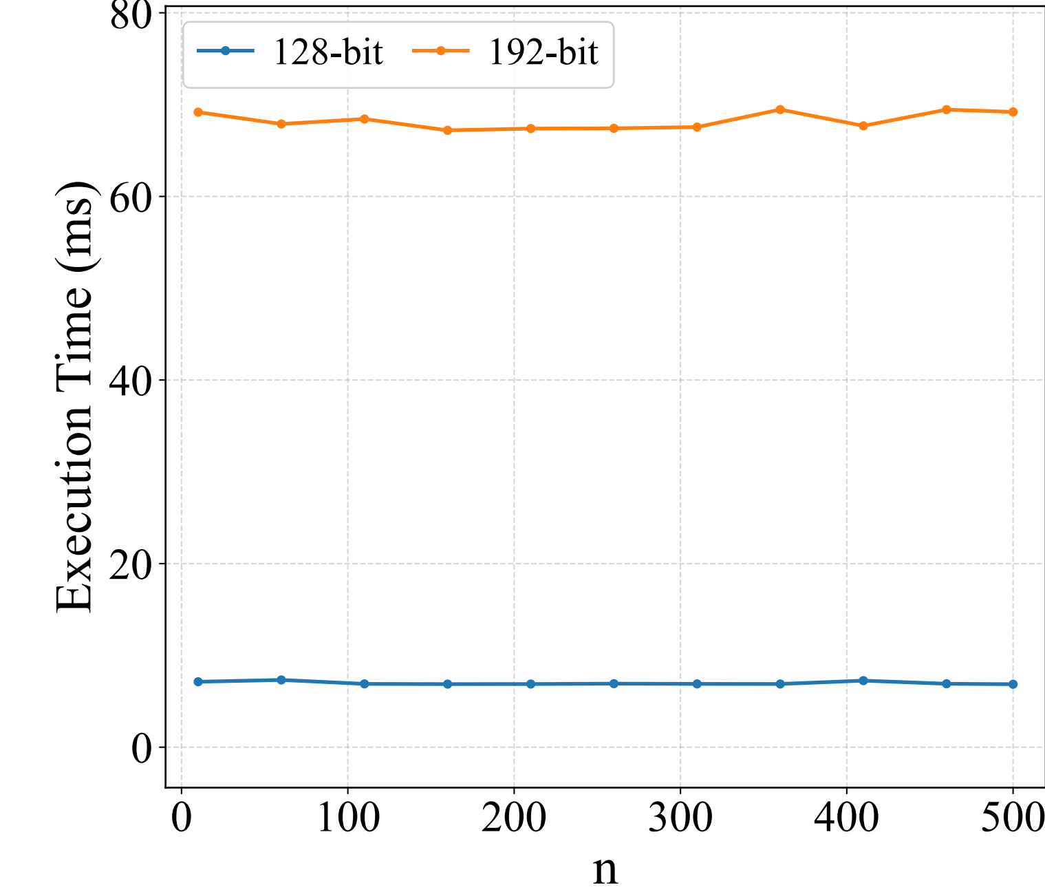
(g) Time Cost of Encap
