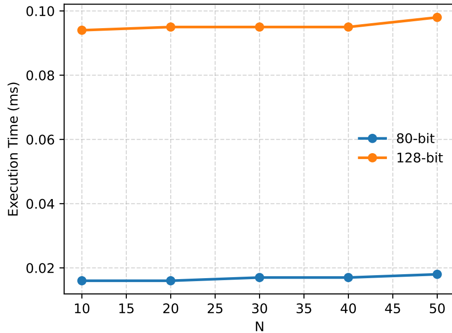
(b) Time Cost of GroupKeyUpdate
