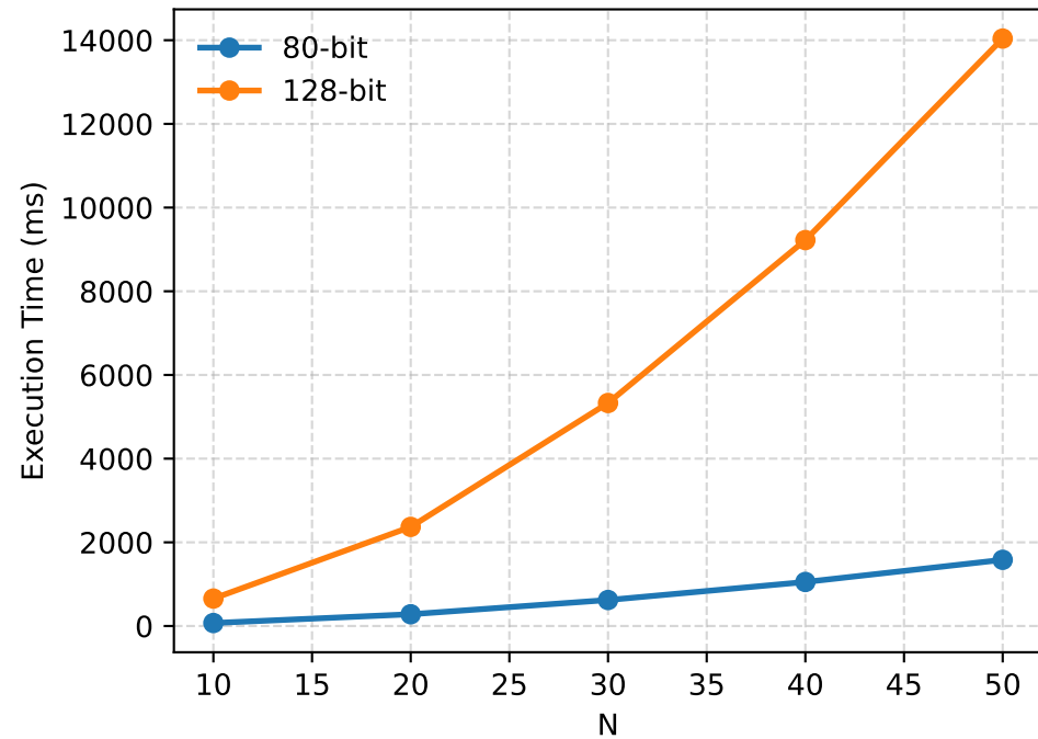
(c) Time Cost of UserGen
