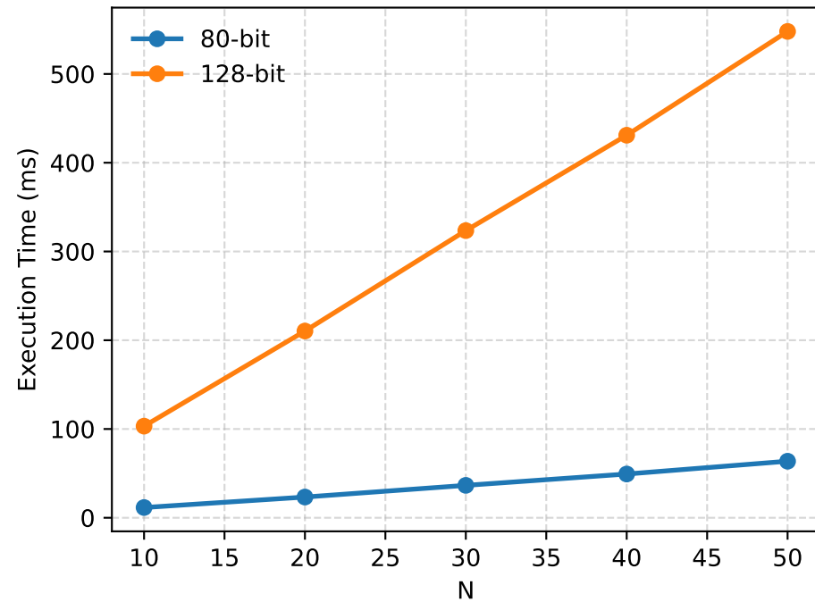
(a) Time Cost of UserKeyUpdate
