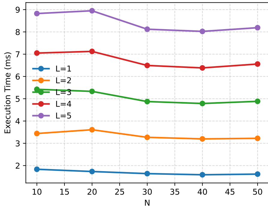
(c) Time Cost of UserKeyUpdate
