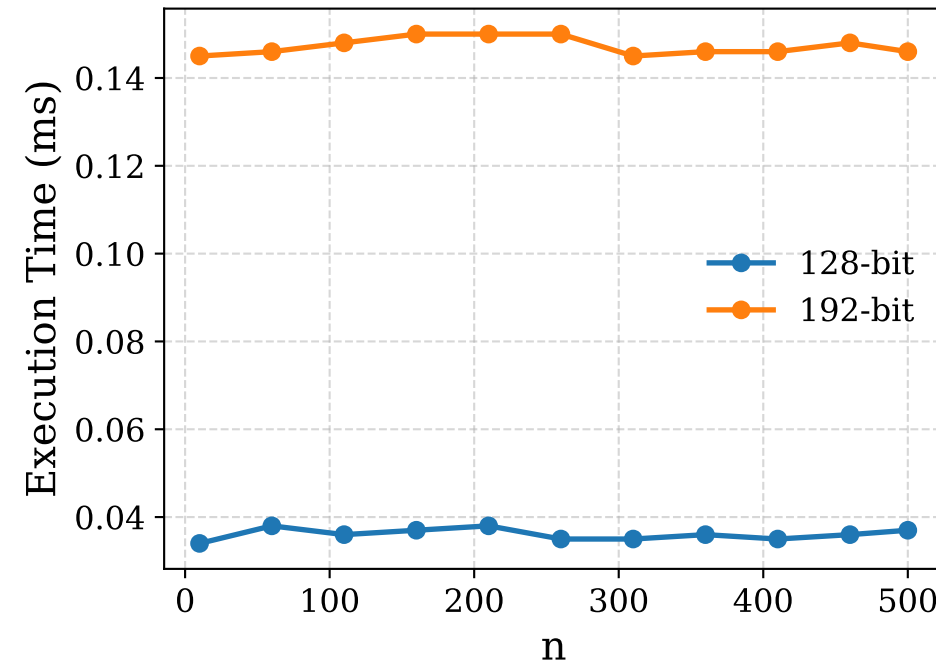
(c) Time Cost of Remove
