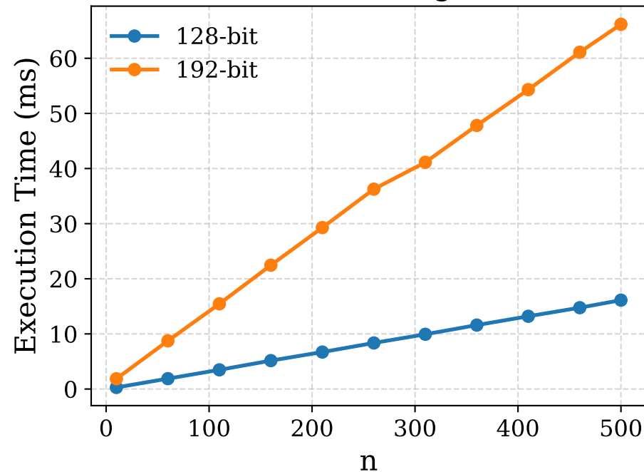
(a) Time Cost of Agreement
