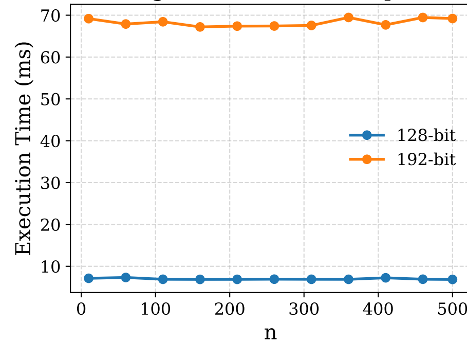
(g) Time Cost of Encap
