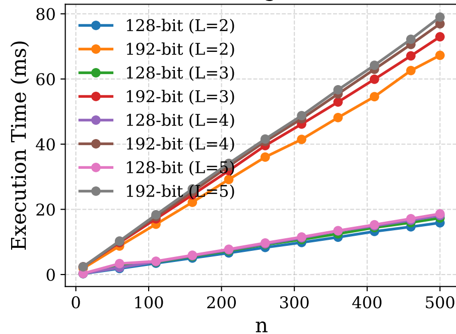
(f) Time Cost of Merge (extended mode)
