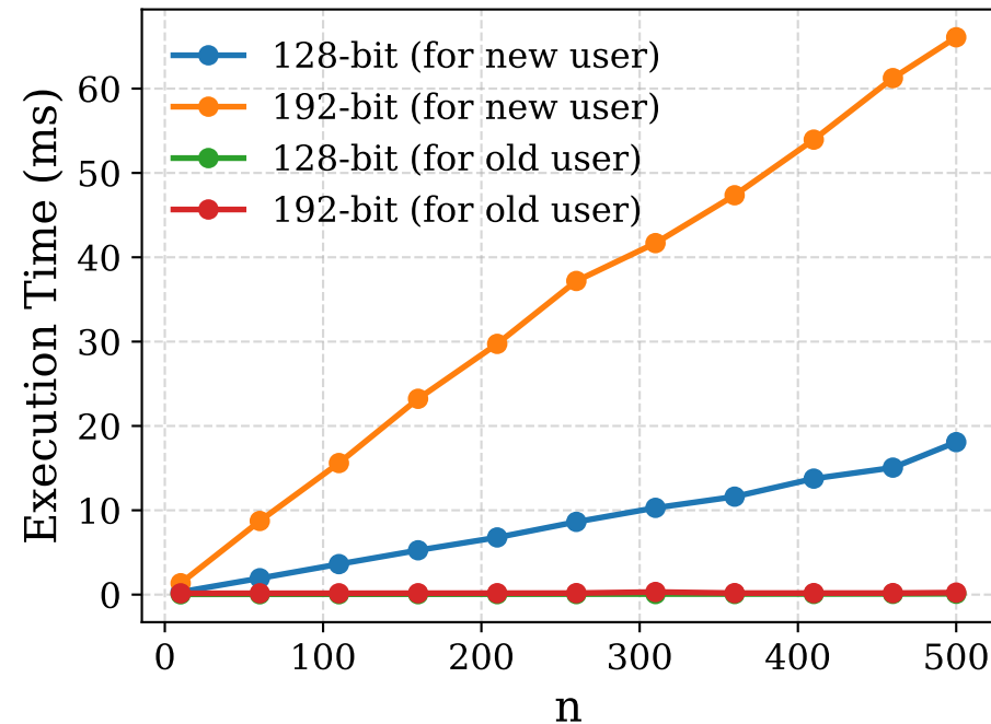
(b) Time Cost of Add
