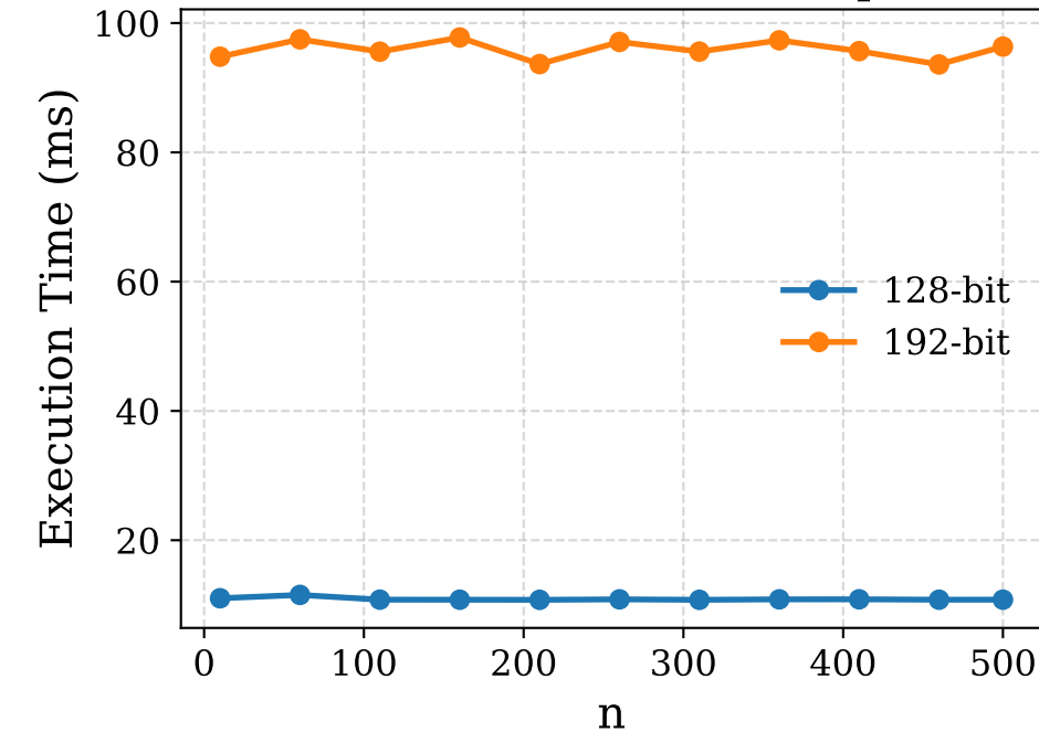
(h) Time Cost of Decap
