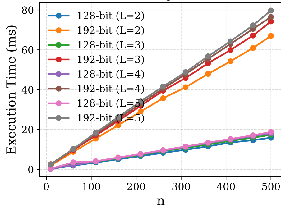
(e) Time Cost of Merge (standard mode)
