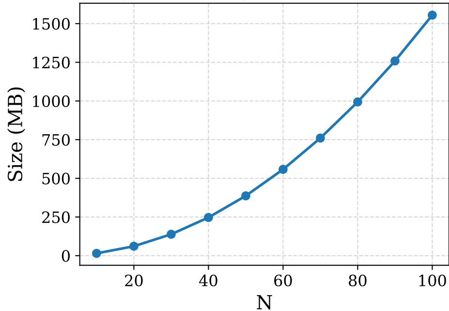
Storage Cost of system parameter/upk
