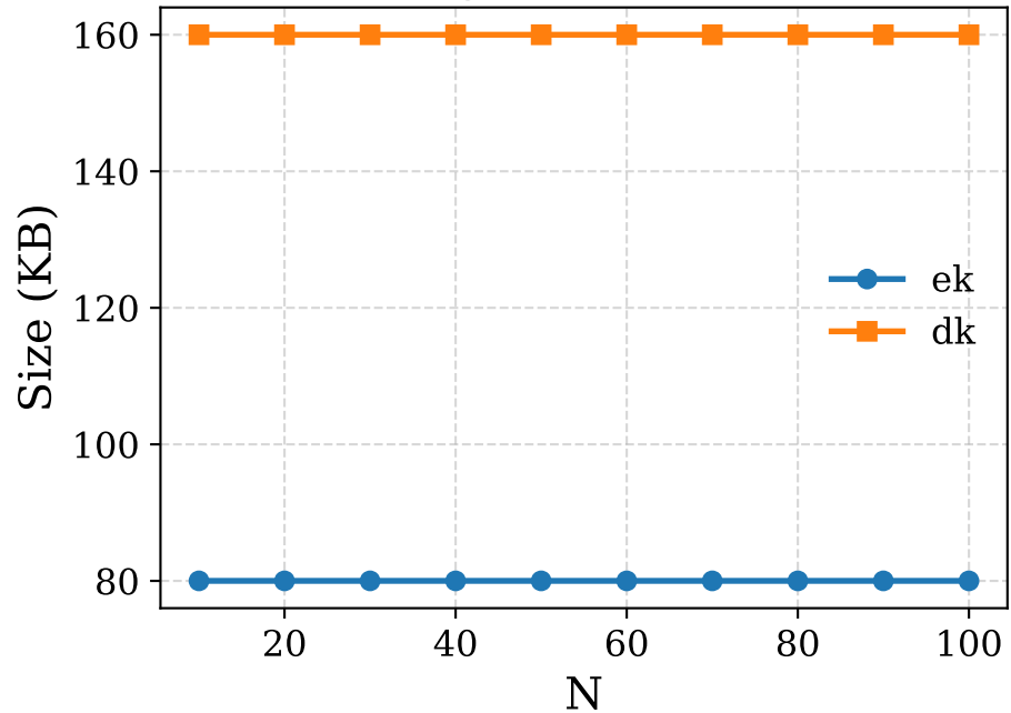
Storage Cost of ek/dk
