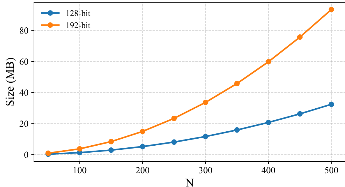
Storage Cost of system parameter/upk
