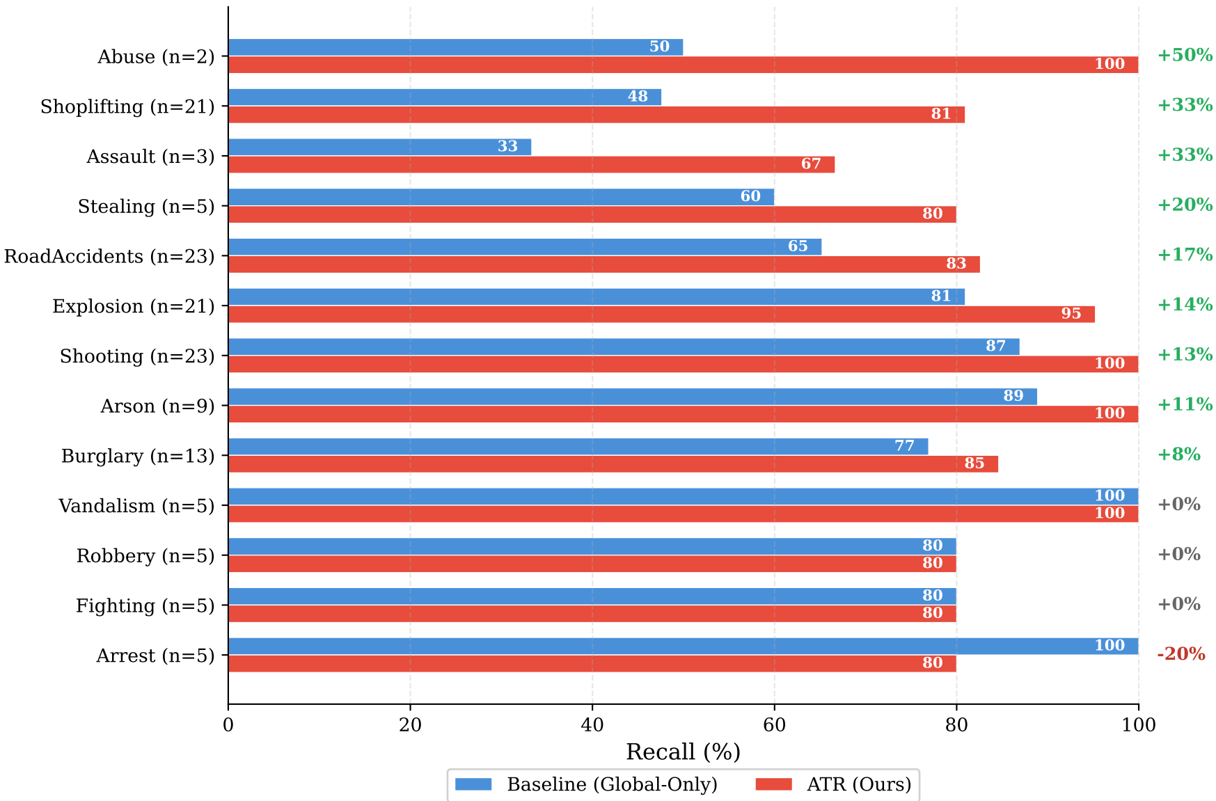
Per-Category Recall: Baseline vs. ATR (4B + Minimal, UCF-Crime Standard Test Set, N=290)
