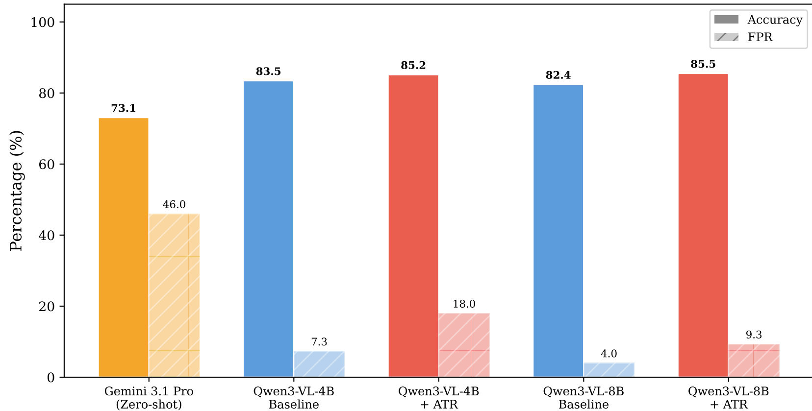
External VLM Baseline: Gemini 3.1 Pro vs ATR (UCF-Crime, N=290)
