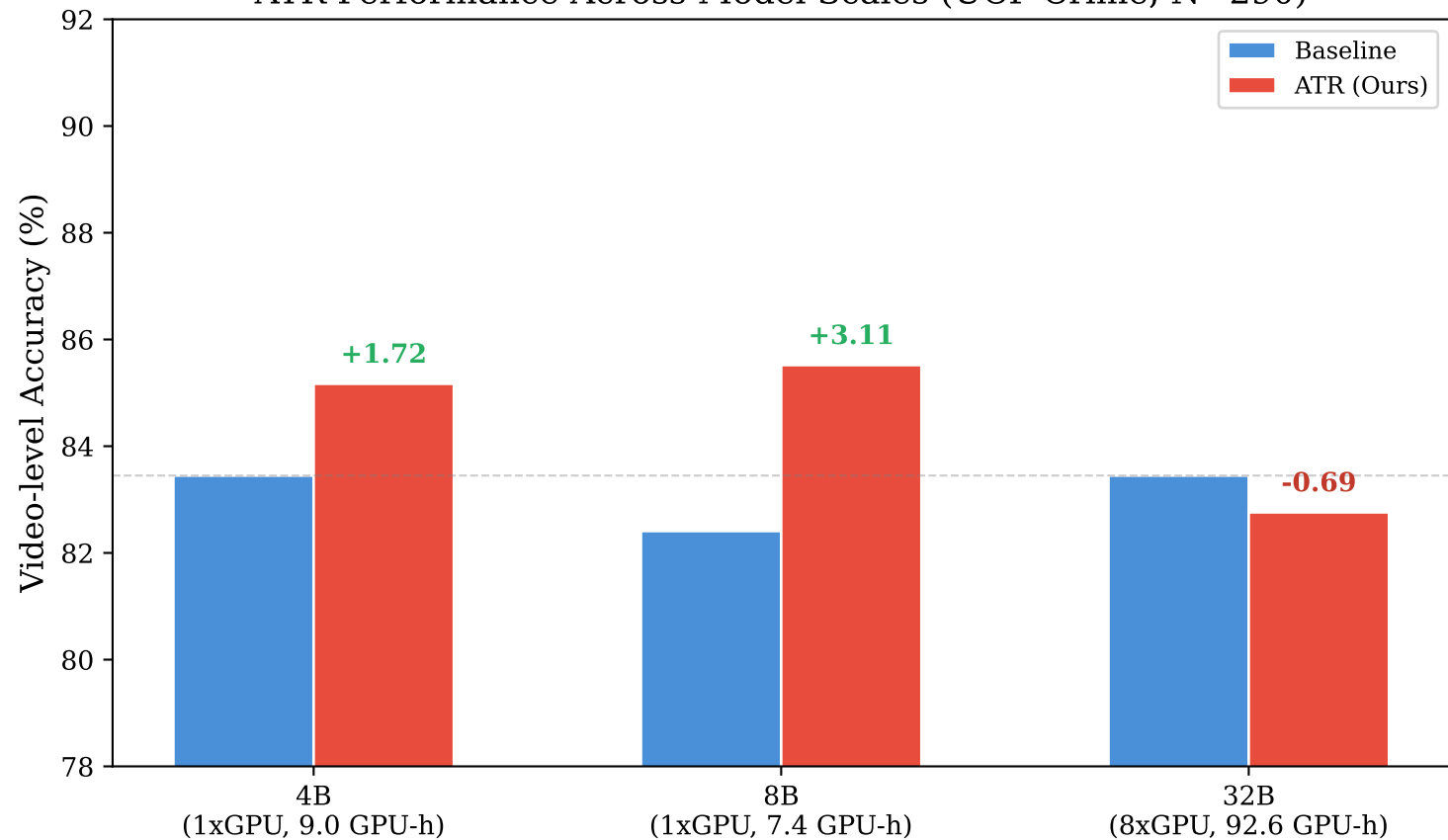
ATR Performance Across Model Scales (UCF-Crime, N=290)
