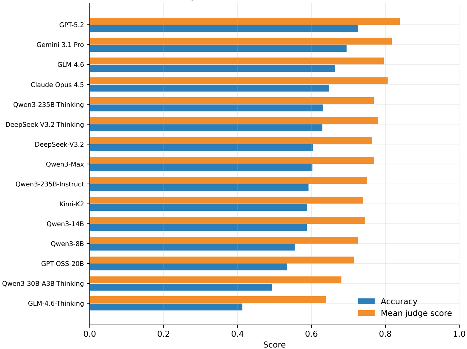
Overall performance across 961 benchmark items
