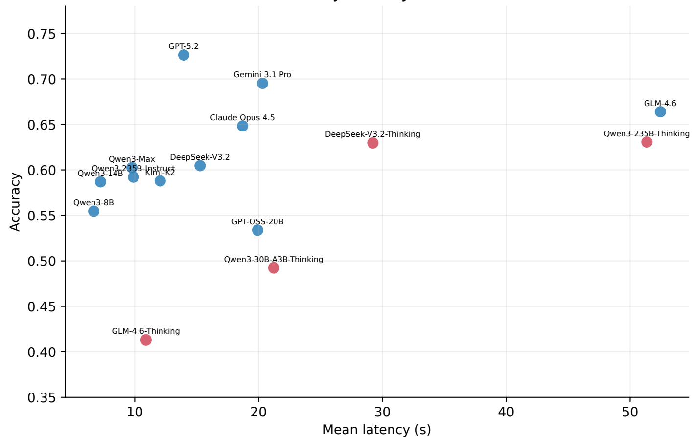
Accuracy--latency trade-off
