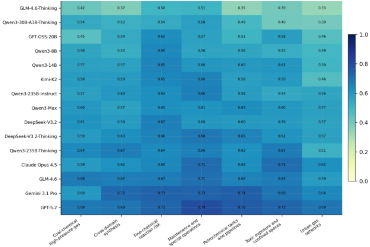
Accuracy by process-safety domain
