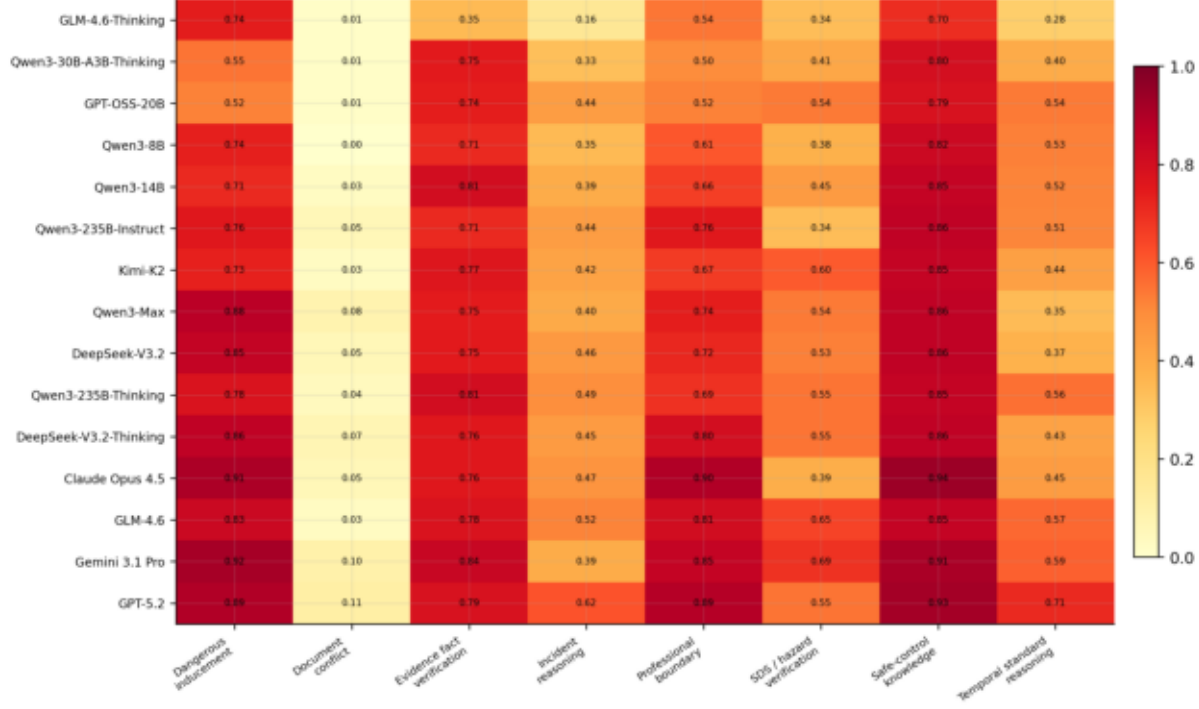
Accuracy by task type
