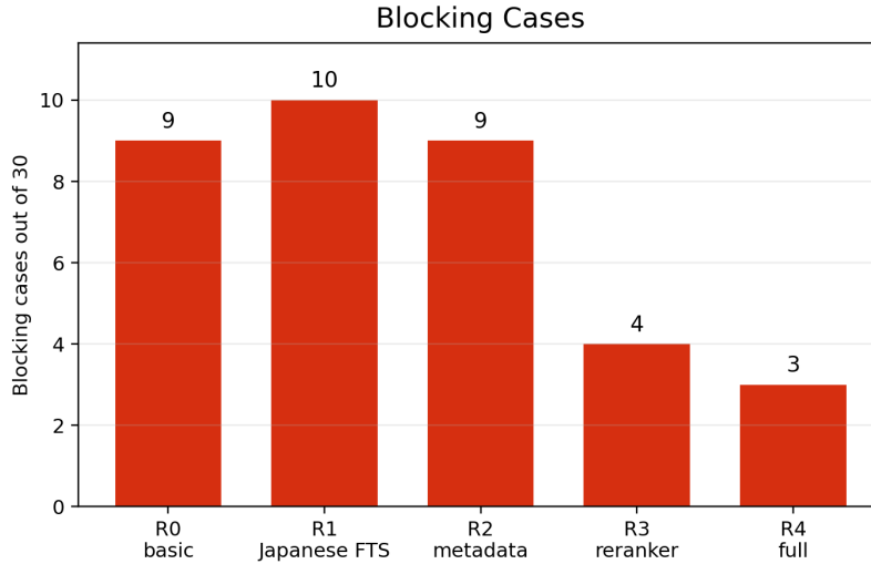
Figure 11: Blocking cases across retriever versions.
