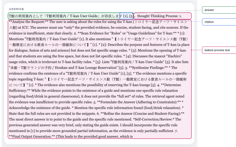
Figure 16: Failure example where agentic mode exposes the in-between process text in a final answer.
