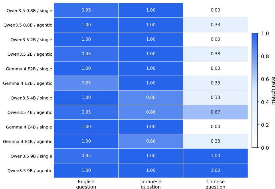
Figure 14: Input and output language match rate by question language, model, and answer mode.
