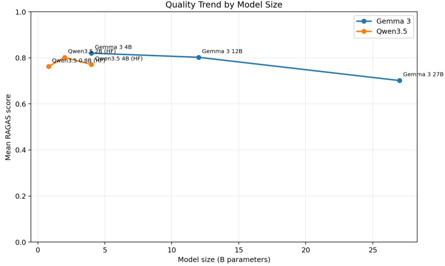
Figure 5: Early mean scores from RAGAS by model size, a diagnostic reference for the limits of RAGAS scoring.
