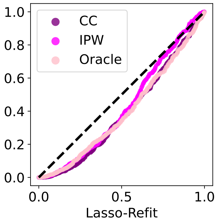
Transformed Studentized Debiased Estimators
