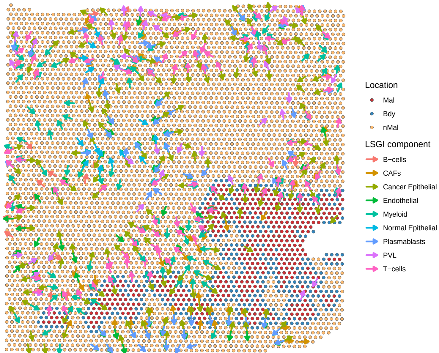
BRCA2 boundary with LSGI cell-component gradients
