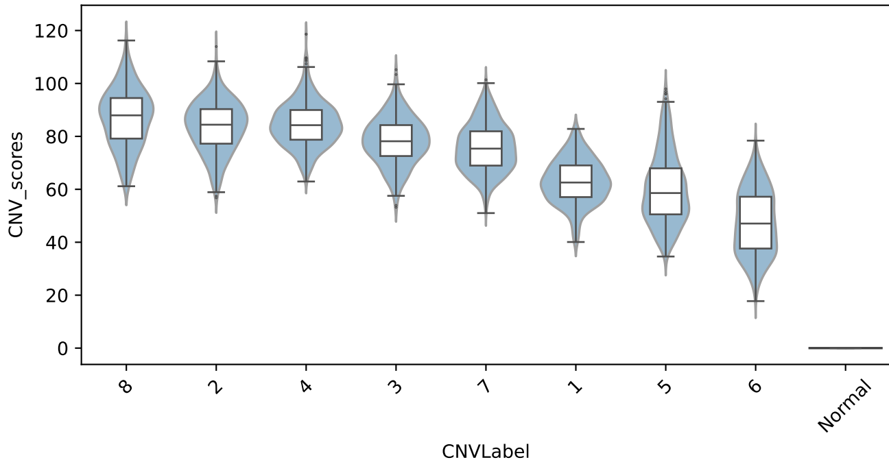
CNV Scores
