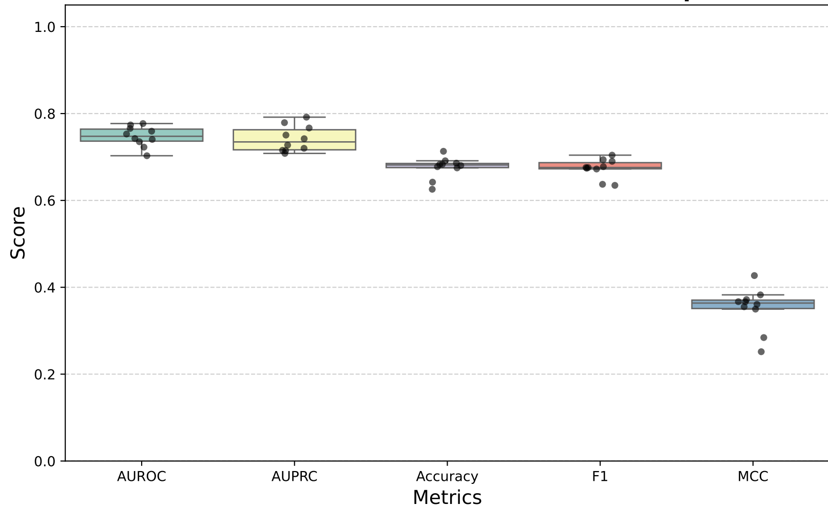
Model Performance across Random Data Splits
