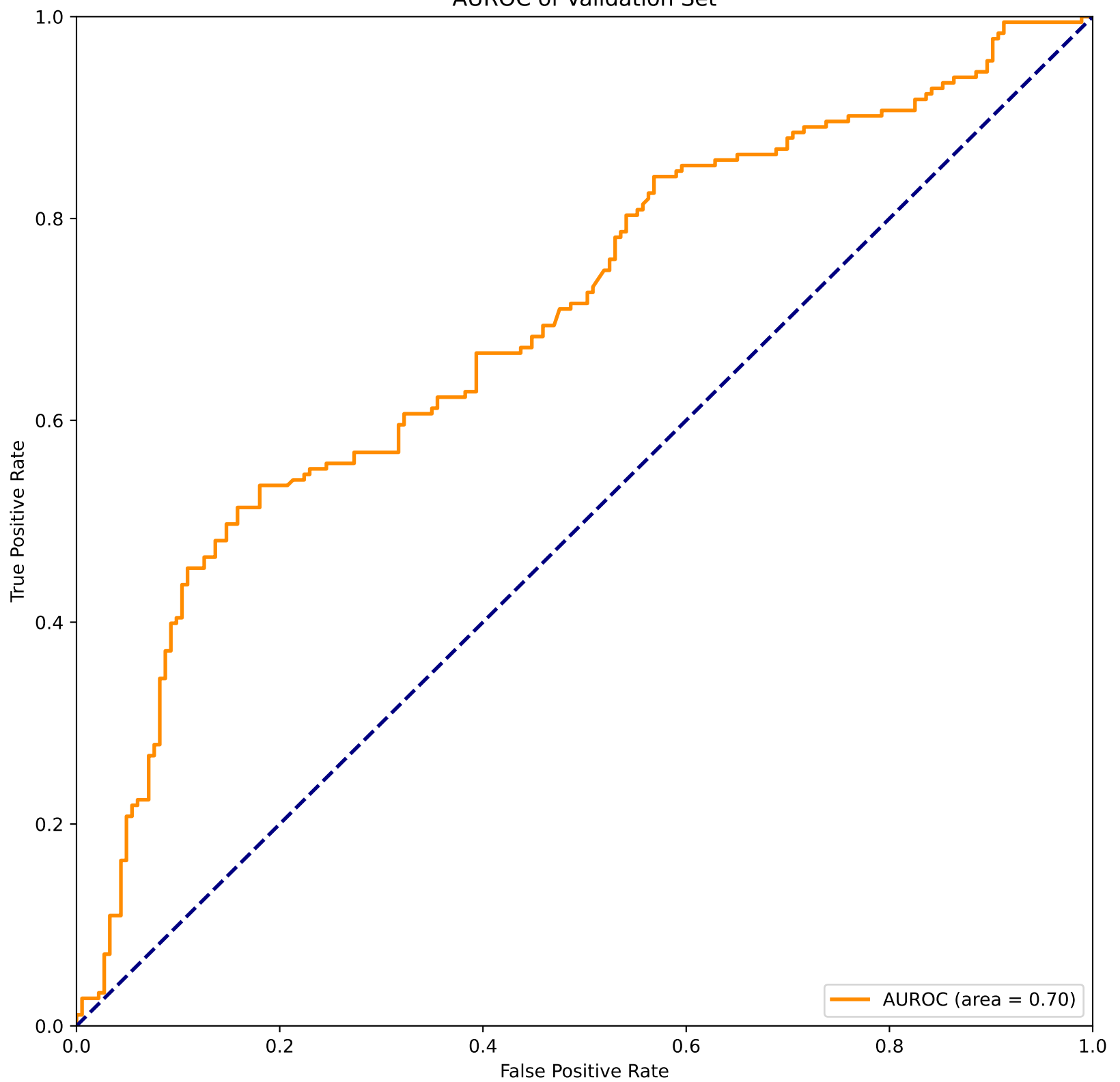
AUROC of Validation Set
