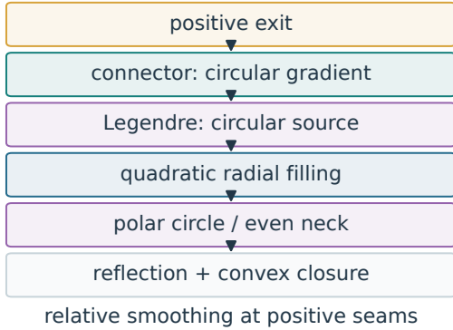
(c) Domain changes in the proof
