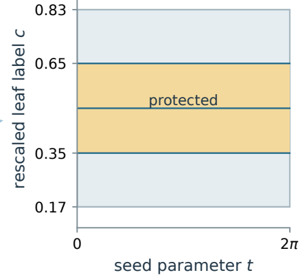
(c) Leaf strip
