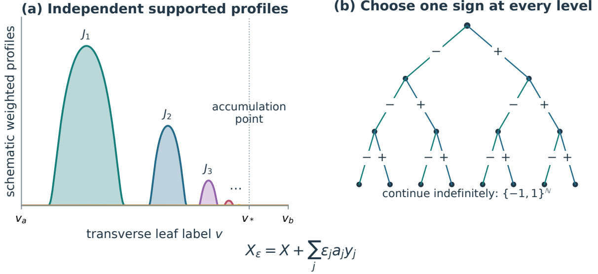
FIGURE 6. The Cantor family as independent sign choices. (a) Schematic weighted test profiles on disjoint transverse intervals J_j \in I accumulating at an interior leaf label. Their supports select disjoint annuli for y_j = \mathcal{V}F_j . The plotted heights only illustrate decay; the proof chooses amplitudes controlling all required C^k norms. (b) Three finite levels show 2, 4, and 8 choices; continuing gives \{-1, 1\}^{\mathbb{N}} with the product topology. Disjoint supports eliminate mixed metric terms, and therefore every branch has the same metric g_X + \sum_j a_j^2 \langle dy_j, dy_j \rangle . Theorem 9.6 proves smooth convergence, tightness, noncongruence, and the embedding into the metric fiber modulo Euclidean isometries. This totally disconnected parameter family is not a continuous isometric flex.
