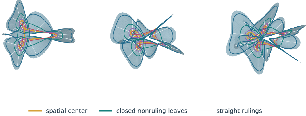
FIGURE 3. Three-, four-, and five-lobed constant-speed ruled bands from the numerical atlas. All axes in each model use equal physical units; the broad strips come from actual ruling widths, not a transverse stretch. Gold is the closed spatial center, colored curved traces show the closed nonruling asymptotic family, and pale straight segments show the ruling family. Traces are overlaid to make the foliation visible. With a = 1 , the nonruling equation is u_r = -\kappa_r u^2/2 , whose reciprocal gains zero over a period. These are illustrations by immersed bands: self-intersections are allowed in the saved models. They are not asserted to be embedded protected cores or completed tight tori.
