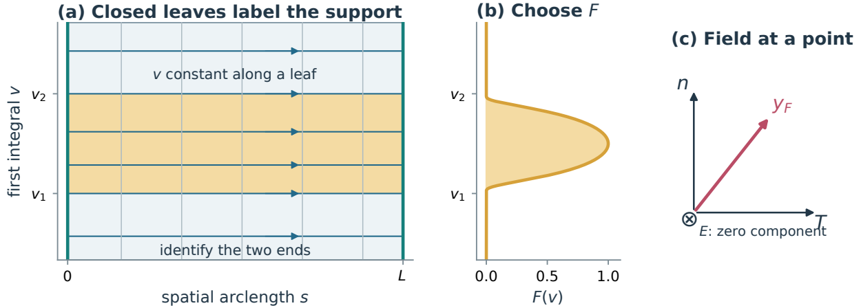
FIGURE 2. The bending map F \mapsto y_F in Theorem 3.3. (a) Cutting the band at s = 0 gives a cylinder diagram with s = 0 and s = L identified. Horizontal curves have constant first integral v ; vertical curves correspond to rulings at fixed s . (b) A smooth function supported between v_1 and v_2 selects the gold subannulus; the field is zero outside it. (c) At each point the exact field has components \langle y_F, T \rangle = \tau u F'(v)/(2\rho) and \langle y_F, n \rangle = u F(v) - (1 - ku)F'(v)/(2\rho) , while \langle y_F, E \rangle = 0 . The displayed arrow illustrates this decomposition; its length and angle are schematic. The characteristic transport equation, not the arrow, establishes the bending identity.
