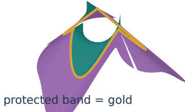
(c) Domain changes in the proof
