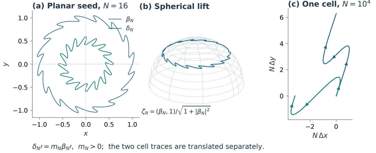
FIGURE 4. The seed formulas (5.3)–(5.5). (a) Blue is \beta_N and teal is \delta_N at N = 16 . (b) The corresponding northern spherical lift \zeta_N . These two panels make corrugation visible; N = 16 is below the sufficient range of Lemma 5.2, so they are illustrations of the formulas. (c) One full cell at N = 10^4 : each curve is translated to its own initial point, and both coordinate differences are multiplied by N . This is an isotropic magnification, not a common placement of the two curves. Arrows show the parameter direction. The oriented tangents agree at corresponding parameters because \delta'_N = m_N \beta'_N with m_N > 0 . The root defining m_N cancels the mixed action, while the covariant initial point closes the partner. The seed estimates are proved in Appendix B.
