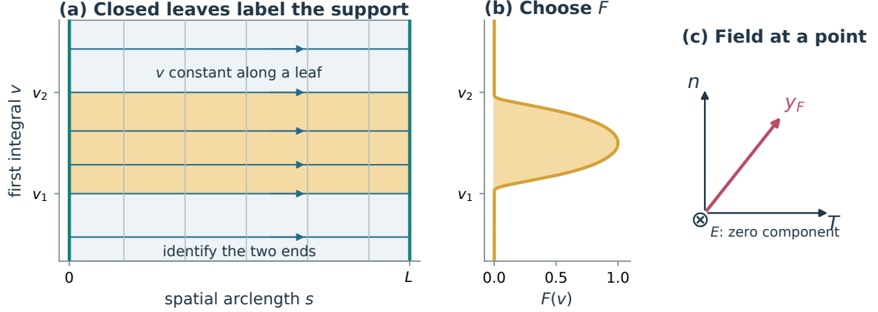
FIGURE 2. The bending map F \mapsto y_F in Theorem 3.3. (a) Cutting a saturated subband at s = 0 gives a cylinder diagram with s = 0 and s = L identified. Horizontal curves have constant first integral v ; vertical curves correspond to rulings at fixed s . (b) For c_b < v_1 < v_2 , a smooth function supported between v_1 and v_2 gives a field supported in the gold subannulus. (c) At each point the exact field has components \langle y_F, T \rangle = \tau u F'(v)/(2\rho) and \langle y_F, n \rangle = u F(v) - (1 - ku)F'(v)/(2\rho) , while \langle y_F, E \rangle = 0 . The displayed arrow illustrates this decomposition; its length and angle are schematic. The characteristic transport equation, not the arrow, establishes the bending identity.
