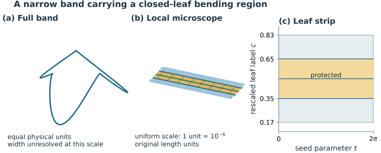
FIGURE 1. The balanced numerical band used by the atlas's saved completion. (a) The complete band, with a protected closed leaf in blue. Its actual width is too small to resolve at this scale. (b) A rigidly rotated, uniformly magnified local patch: one displayed length unit equals 10^{-6} original units. Gold marks the unchanged closed-leaf region; blue and teal curves are its asymptotic leaves, and the short transverse lines are straight rulings there. (c) An unrolled parameter diagram, rather than a physical projection, with protected levels 0.35 \leq c \leq 0.65 and the two ends identified. This saved balanced numerical example illustrates the construction; the analytic existence argument is Lemma 5.2 and Theorem 5.5.
