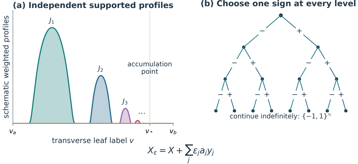
FIGURE 6. The Cantor family as independent sign choices. (a) Schematic weighted test profiles on disjoint transverse intervals J_j \in I accumulating at an interior leaf label. The associated fields y_j = \mathcal{Y}F_j have supports lying in disjoint annuli. The plotted heights only illustrate decay; the proof chooses amplitudes controlling all required C^k norms. (b) Three finite levels show 2, 4, and 8 choices; continuing gives \{-1, 1\}^{\mathbb{N}} with the product topology. Disjoint supports eliminate mixed metric terms, and therefore every branch has the same metric g_X + \sum_j a_j^2 \langle dy_j, dy_j \rangle . Theorem 9.6 proves smooth convergence, tightness, noncongruence, and the embedding into the metric fiber modulo Euclidean isometries. This totally disconnected parameter family is not a continuous isometric flex.
