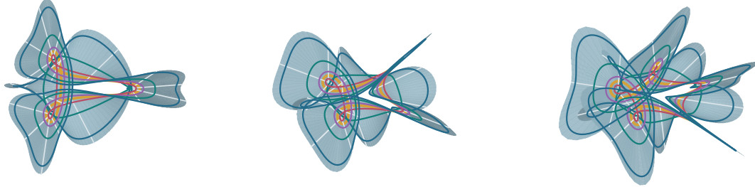
(a) Three lobes
