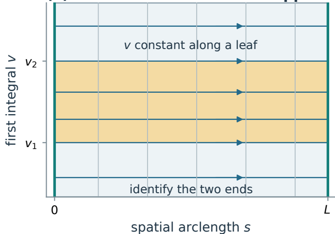
(a) Closed leaves label the support
