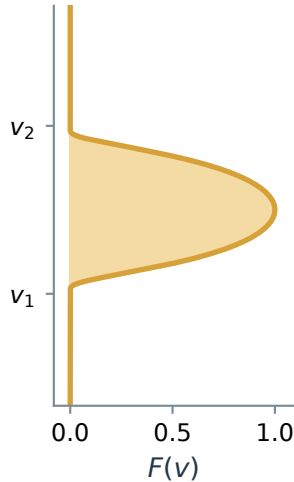
(b) Choose F
