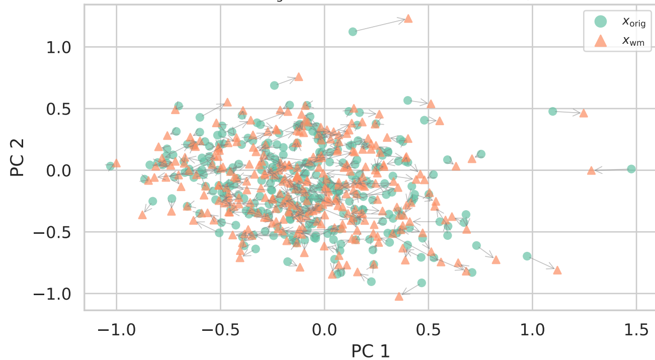
(b) Watermark shift in PCA space (arrows: x_{\text{orig}} \rightarrow x_{\text{wm}} , 300 WM nodes sampled)
