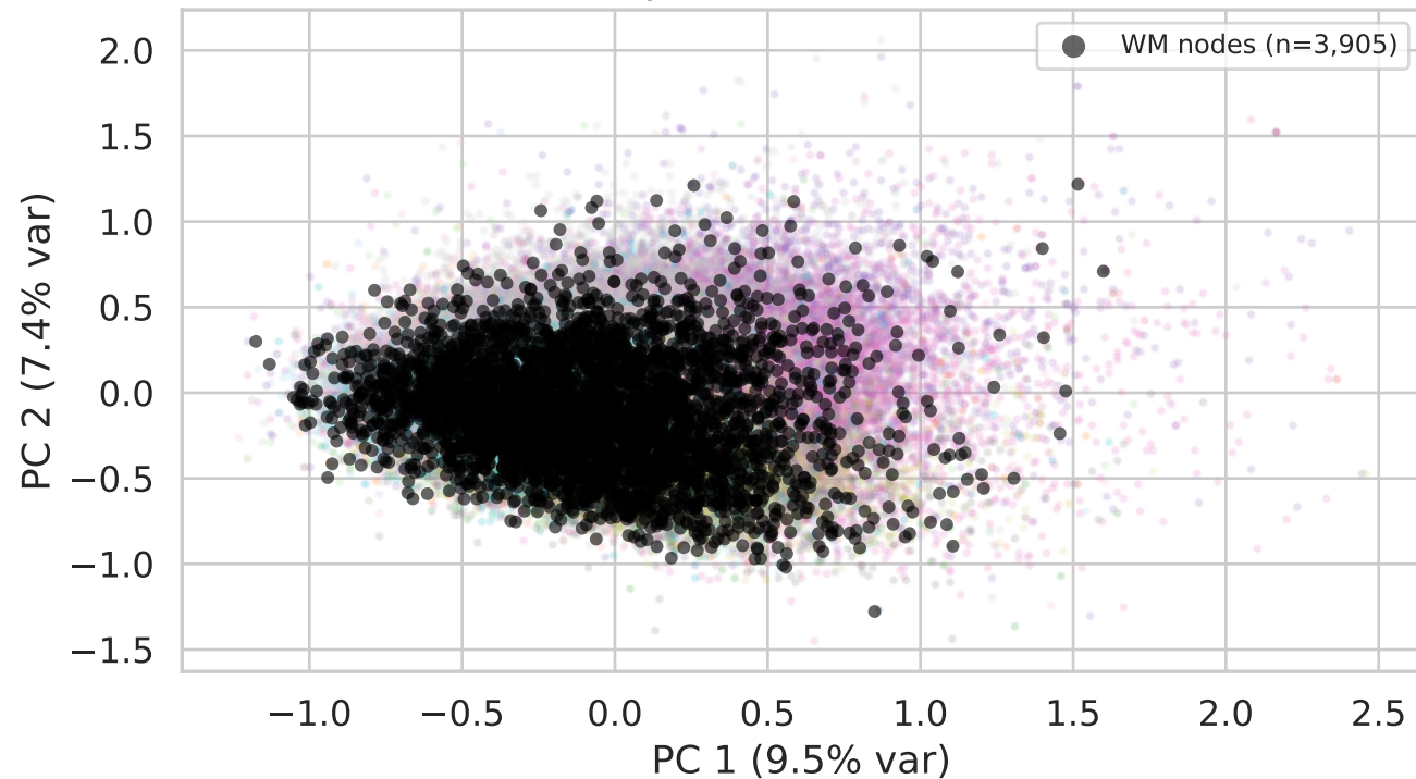
(a) PCA of x_{\text{orig}} (coloured by class, WM nodes in black)
