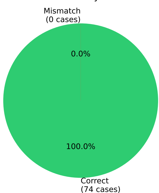
Overall Accuracy: 100.0%
