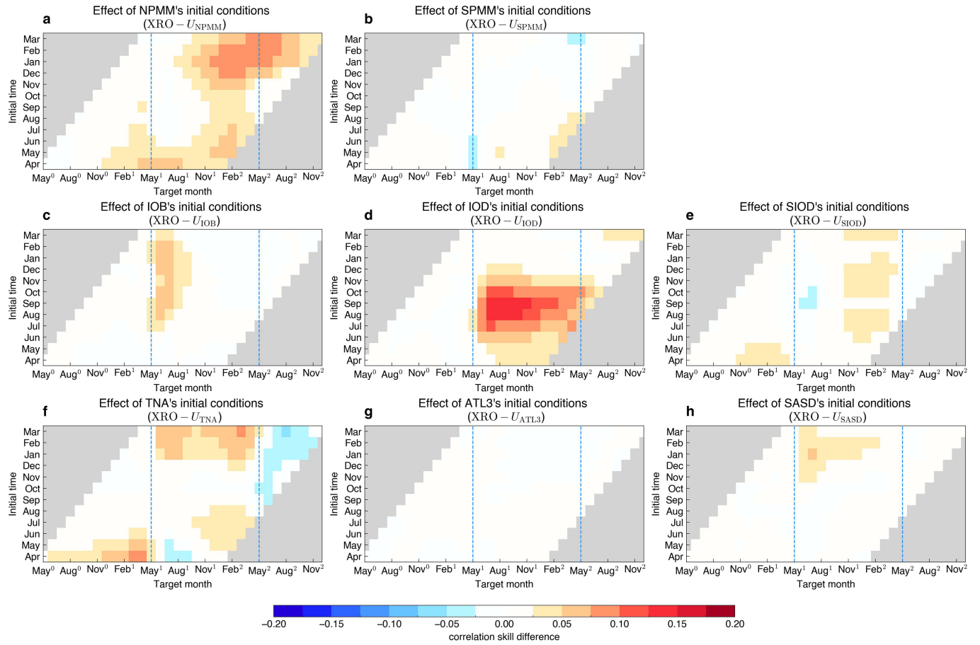
Extended Data Fig. 5 | Contribution of each climate mode's initialization to ENSO correlation skill. Shown is the forecast skill difference of the Niño3.4 SSTa index, as a function of initial time and target month, between the control
