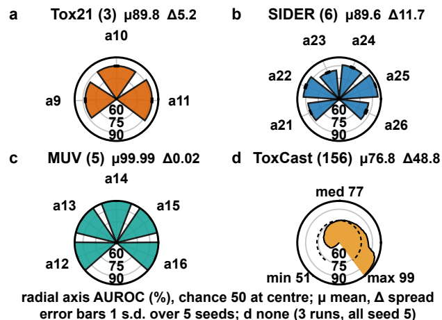
Figure 10: Per-assay AUROC on the meta-test split. Each petal represents one assay, and the radial axis begins at chance performance.
