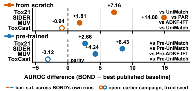
Figure 8: Gain of BOND over the strongest published baseline for each dataset and training protocol. Each interval represents the run-to-run variation of BOND rather than an interval for the difference between means.
