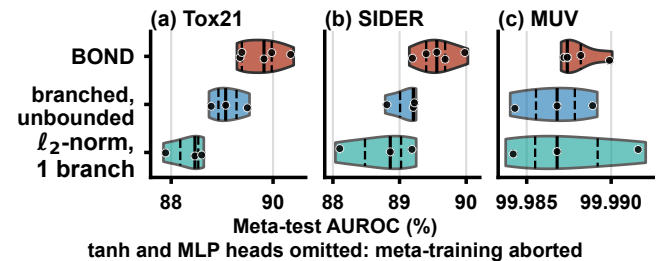
Figure 9: Distribution of the reported metric across feature maps. Violins show the pooled per-seed distributions, horizontal dashes indicate quartiles, and dots represent individual seeds.
