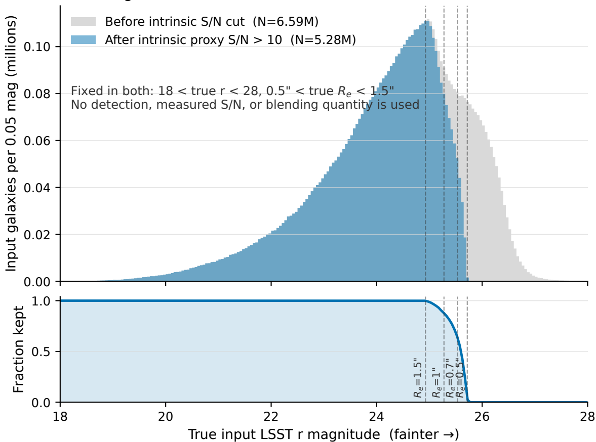
True-magnitude distribution before and after the V2.1 intrinsic S/N cut
