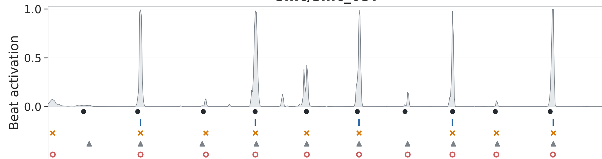
(a) Clear periodicity: CASM improves smc/smc_037
