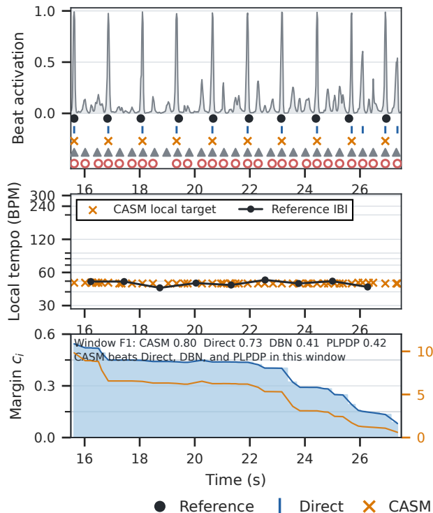
(a) Clear periodicity: CASM wins across decoders Beat This / SMC OOF · smc/smc_001
