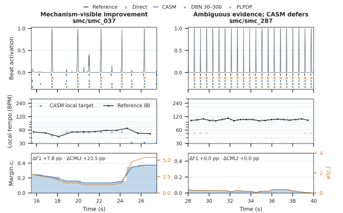
Fig. 1. CASM behaviour on held-out Beat This activations from SMC. Clear local periodicity recovers weak activation-supported beats (left), whereas ambiguous competing periods make CASM defer to Direct (right). Reference IBI is shown only for interpretation.
