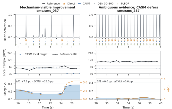
Fig. 1. CASM behaviour on held-out Beat This activations from SMC. Clear local periodicity recovers weak activation-supported beats (left), whereas ambiguous competing periods make CASM defer to Direct (right). Reference IBI is shown only for interpretation.
