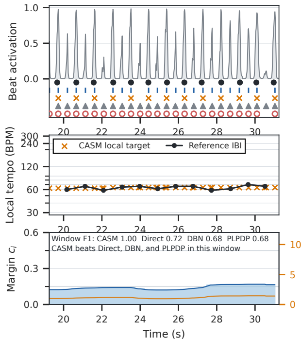
(a) Clear periodicity: CASM wins across decoders Beat This / SMC OOF · smc/smc_036
