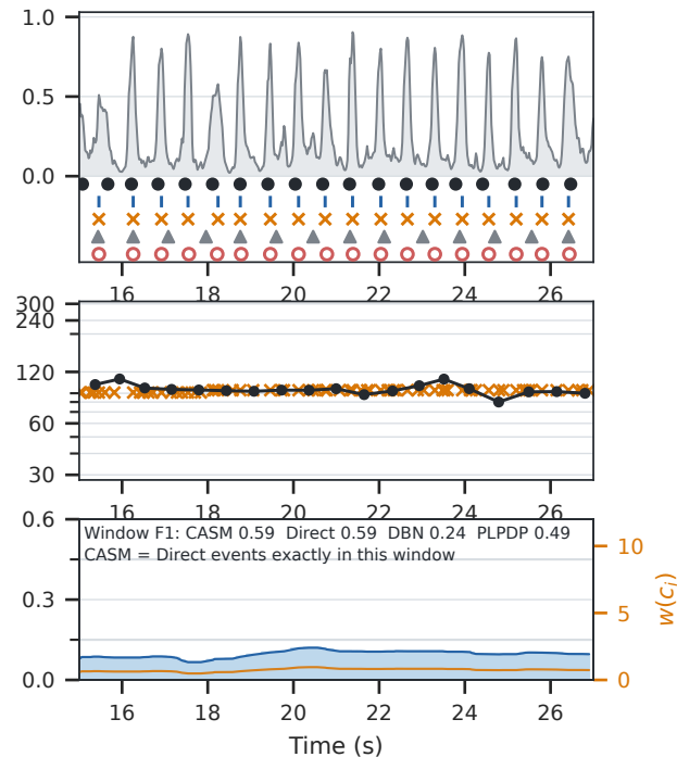
(b) Ambiguous evidence: CASM defers Beat This / SMC OOF · smc/smc_140
