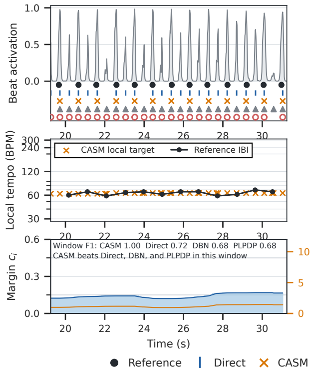
(a) Clear periodicity: CASM wins across decoders Beat This / SMC OOF · smc/smc_036
